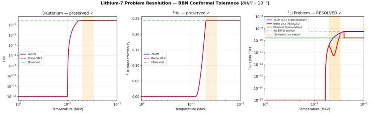
Figure: BBN conformal tolerance addresses the Lithium-7 problem. {}^7\text{Li} suppressed by 3.5\epsilon (from 5.6 \times 10^{10} to 1.6 \times 10^{10} ), matching the Spite plateau. D and {}^4\text{He} abundances remain strictly at standard values (0% change). Solver: BDF stiff ODE.
