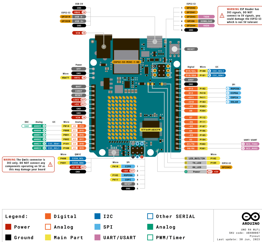
Pinout for UNO R4 WiFi.
