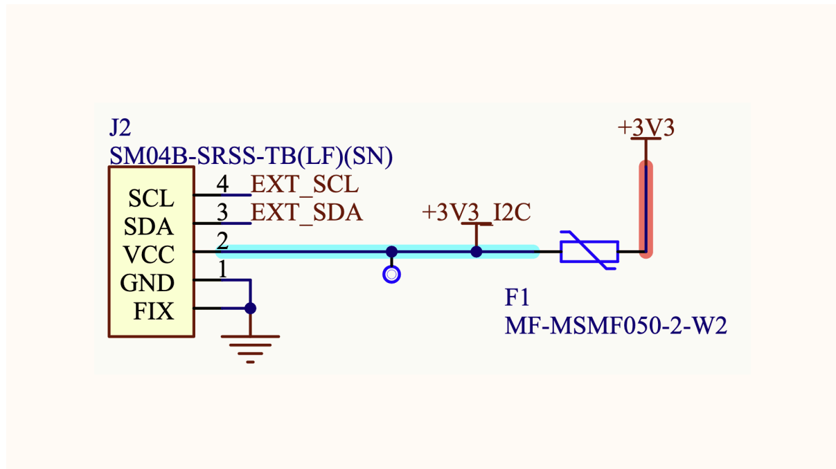
I2C Qwiic connector.
