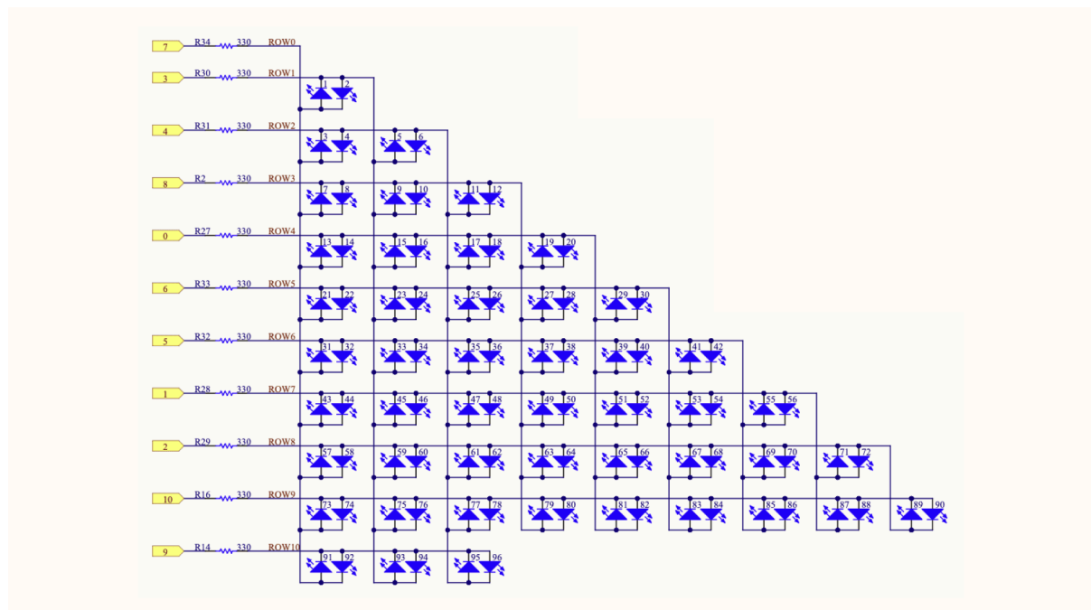
LED matrix schematics.
