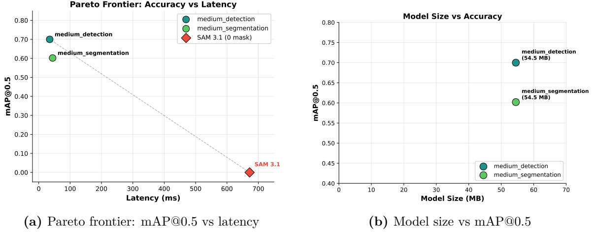
Figure 7: Accuracy–efficiency trade-off for medium models.
