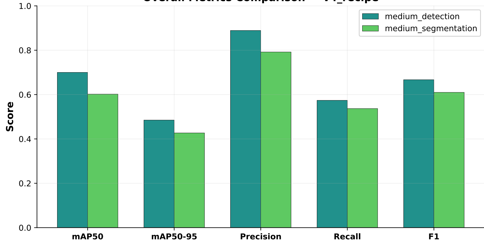
Overall Metrics Comparison — v4_recipe
