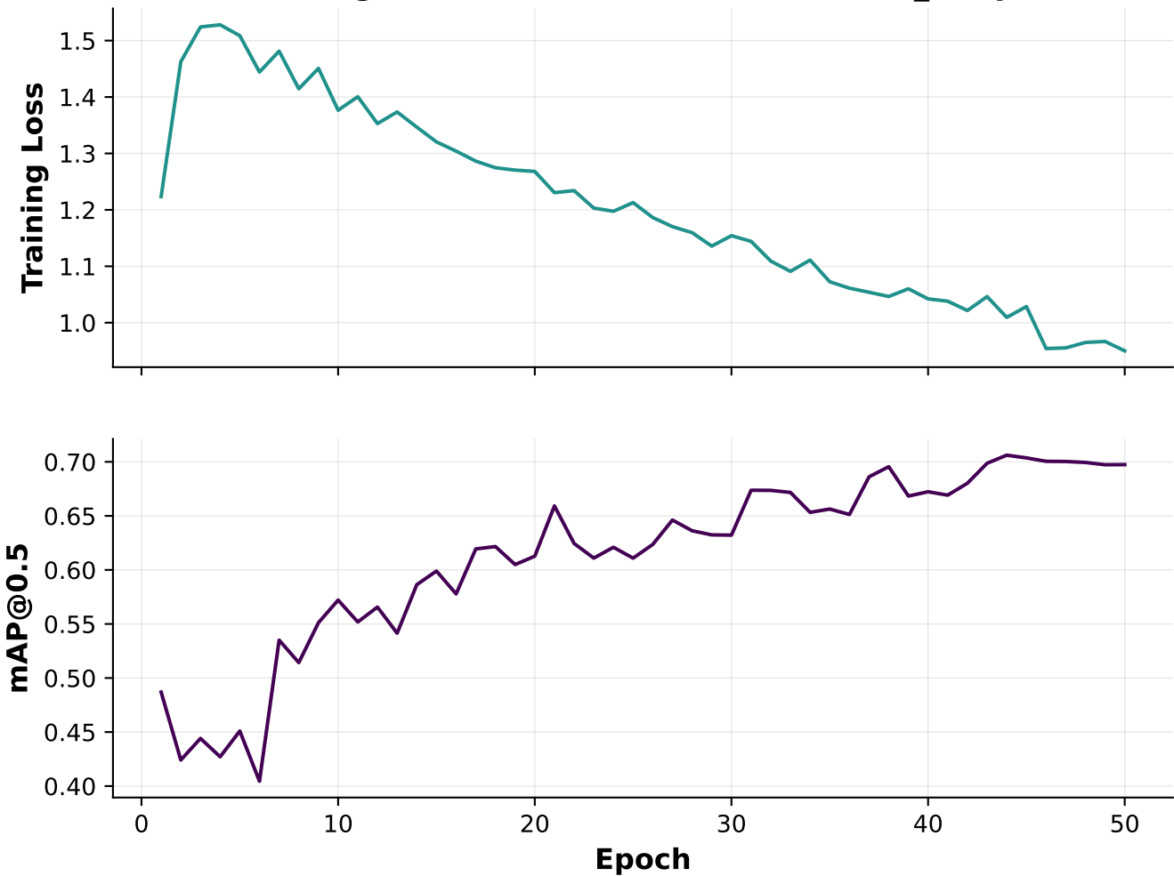
Training Curves — YOLO26m detect (v4_recipe)
