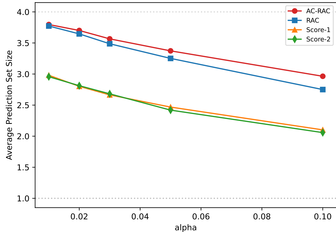
(a) Prediction Set Size
