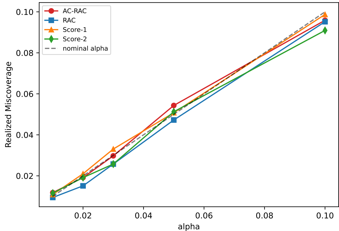
(b) Marginal Miscoverage
