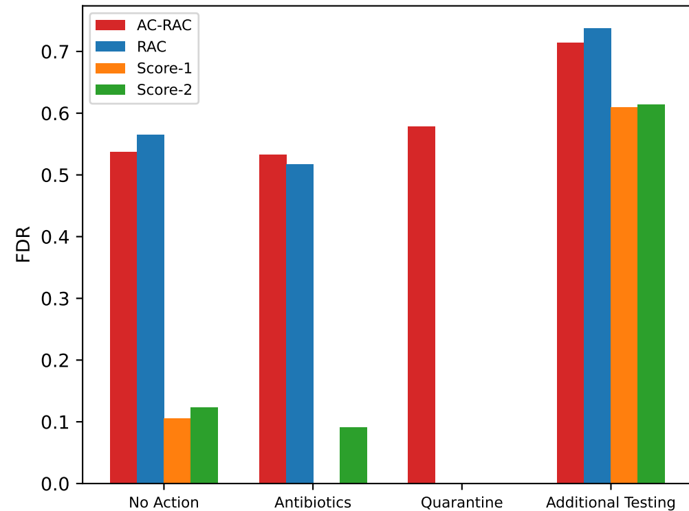
(c) Per-Action FDR
