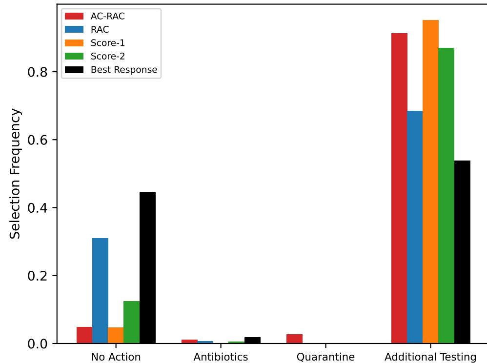
(a) Action Selection Frequency
