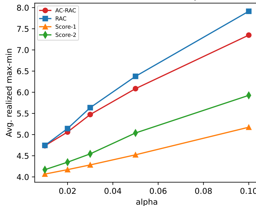
MovieLens Max-Min Utility
