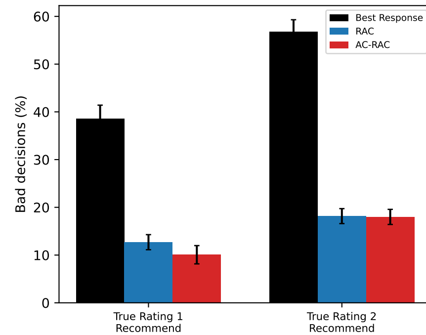
MovieLens Critical Decisions
