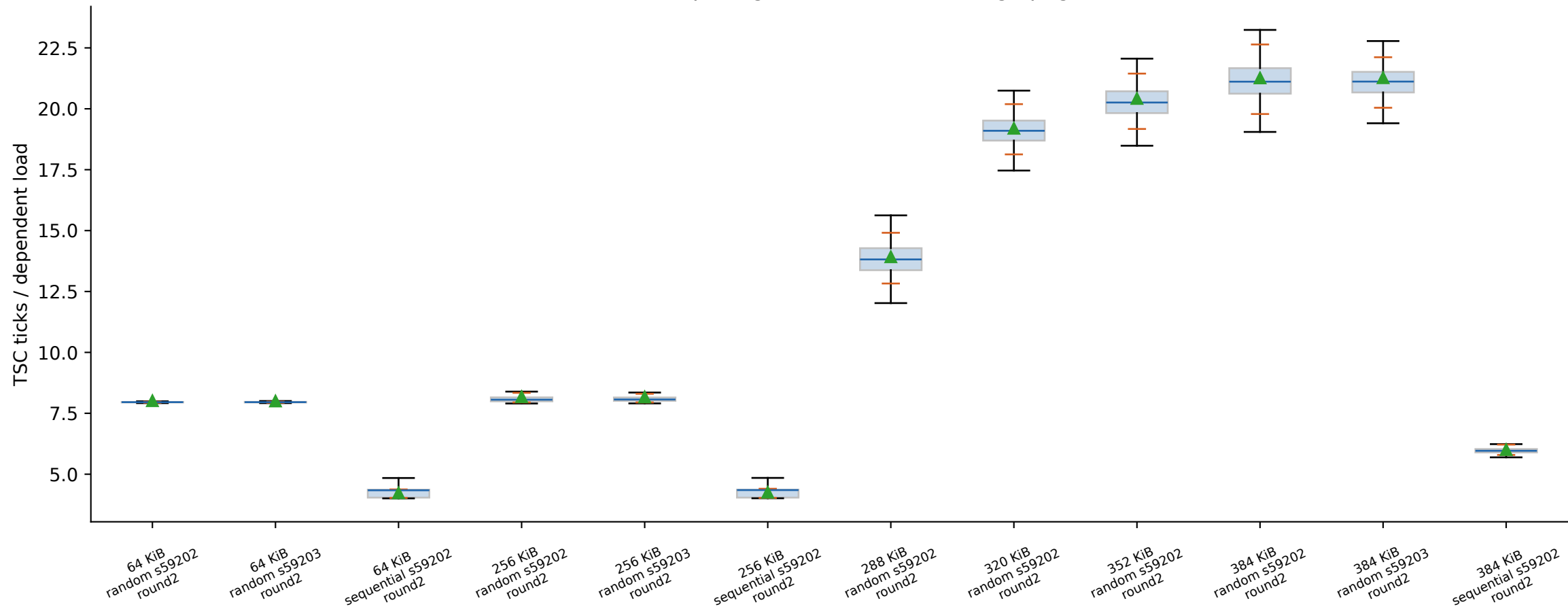
crux: 64 B spacing, 256 loads/batch, huge pages
