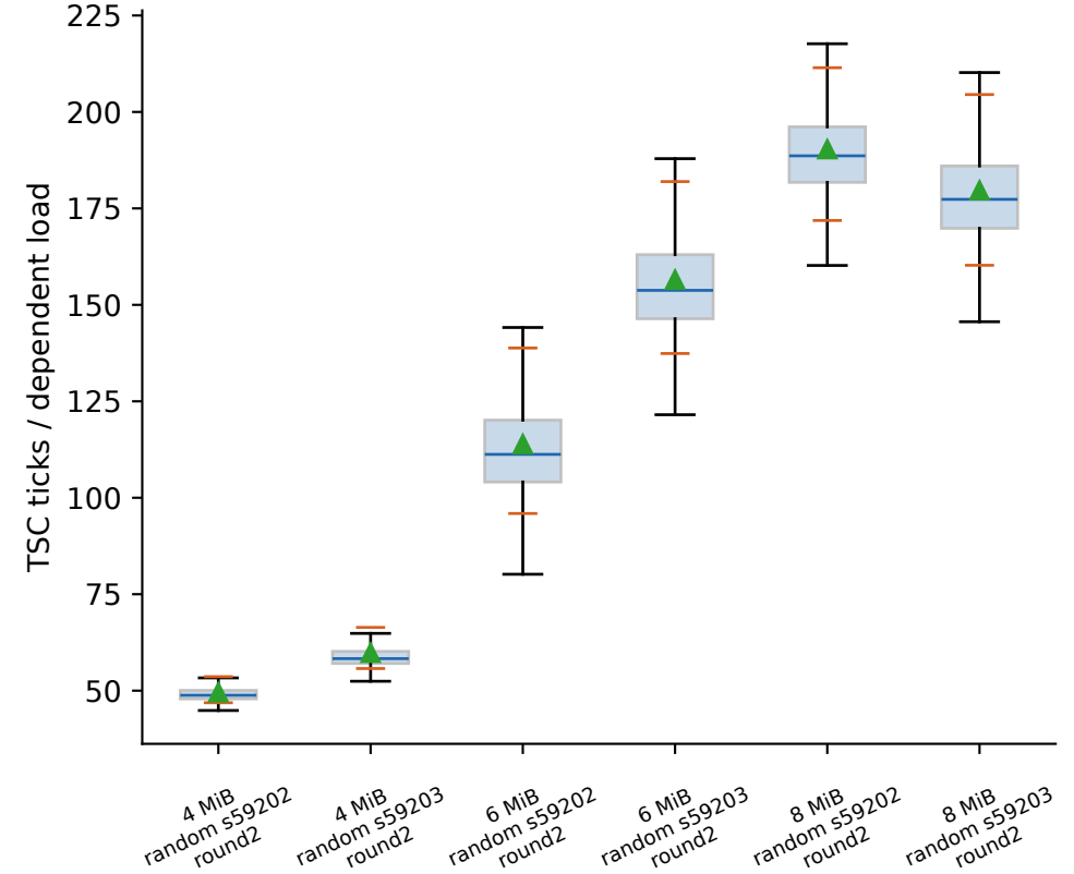
charnwood: LLC effective transition
