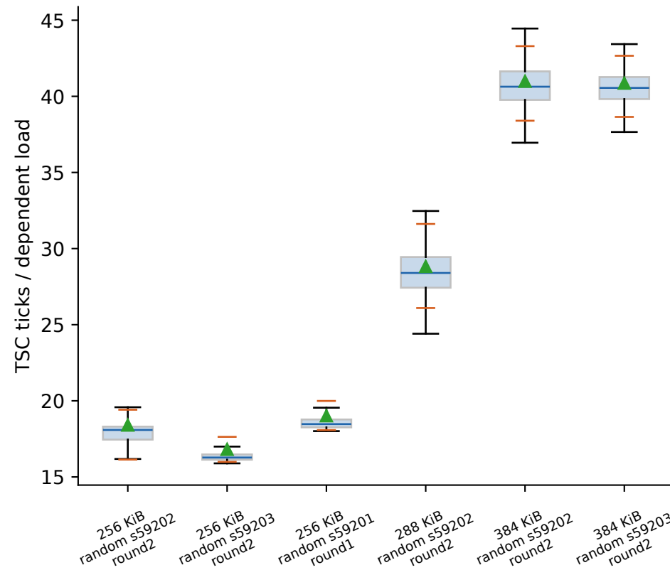
charnwood: L2
