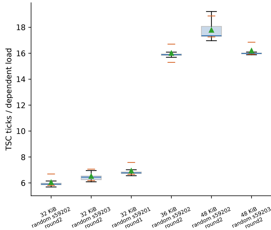
charnwood: L1D
