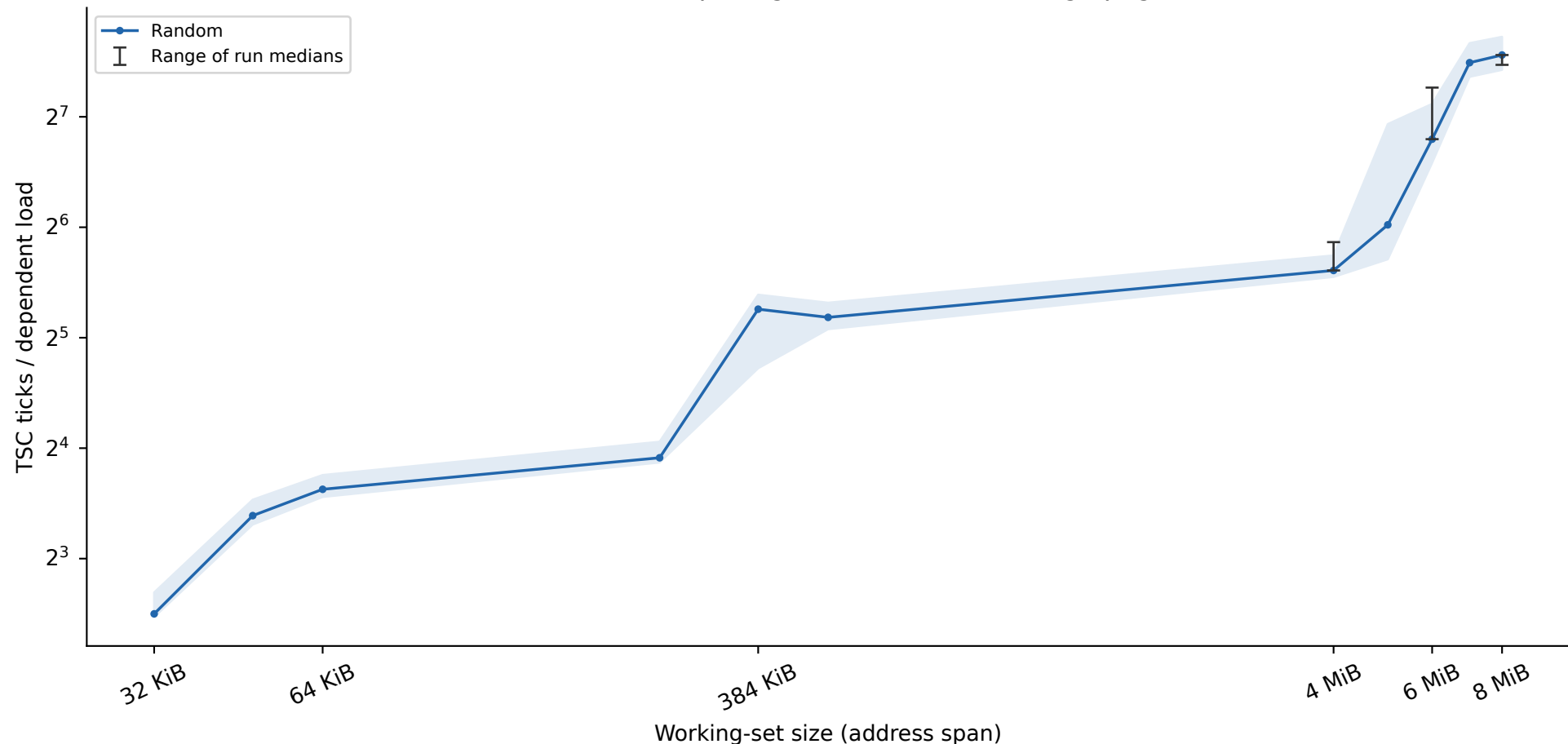
charnwood: 8 B spacing, 256 loads/batch, huge pages
