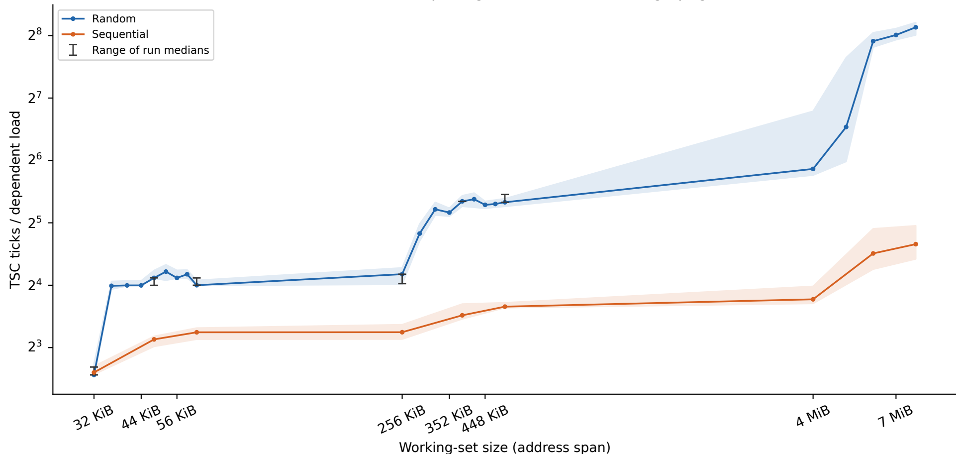
charnwood: 64 B spacing, 256 loads/batch, huge pages
