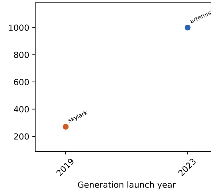
l1c misses
