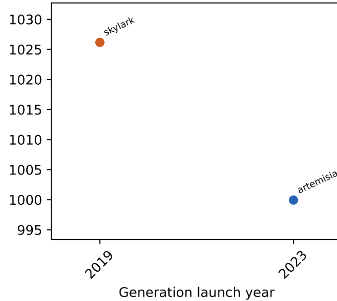
l1c loads
