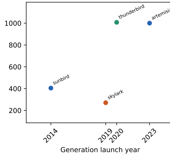
l1c misses
