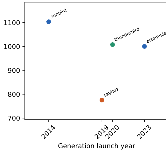
l1c loads
