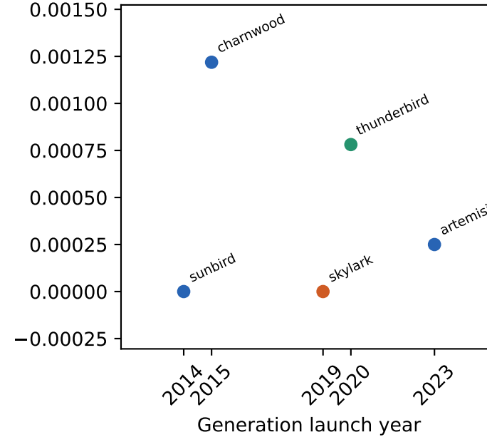
l1c misses
