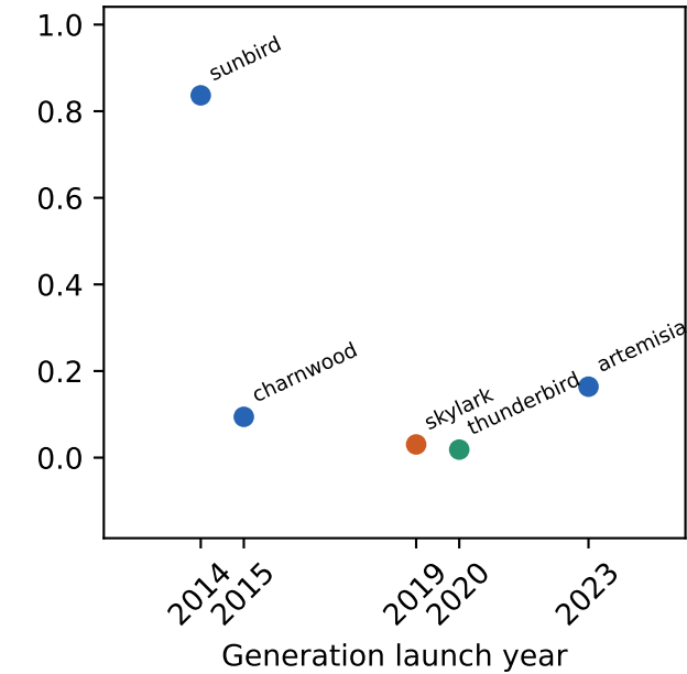
dtlb misses
