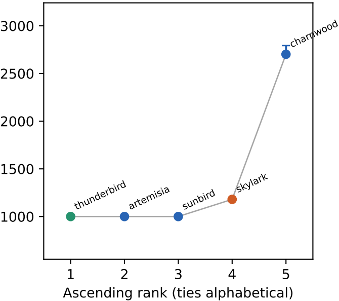
llc loads
