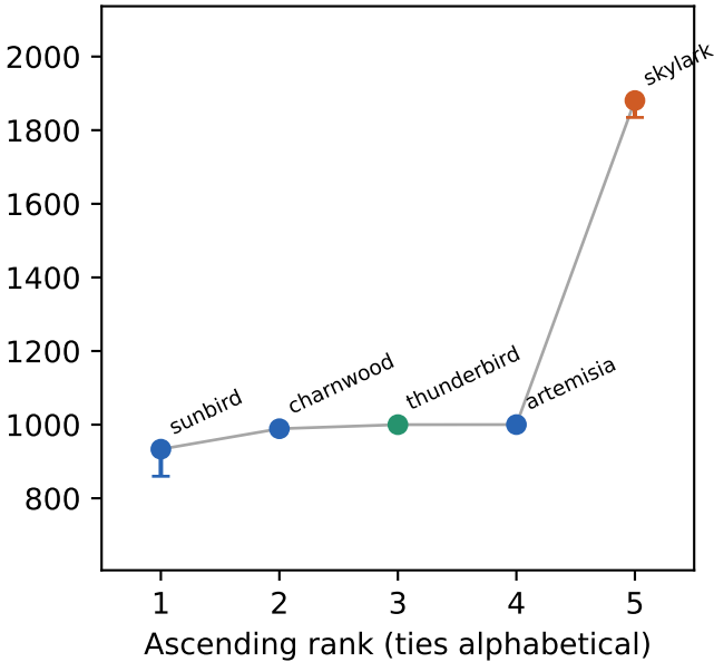
llc misses
