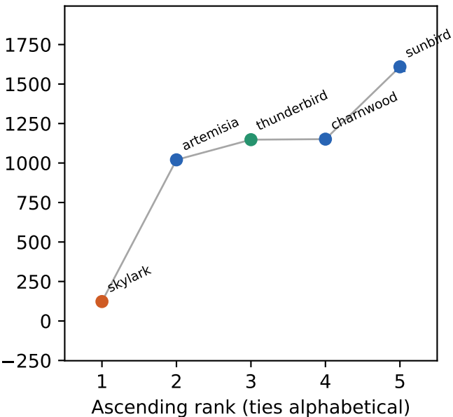
llc loads
