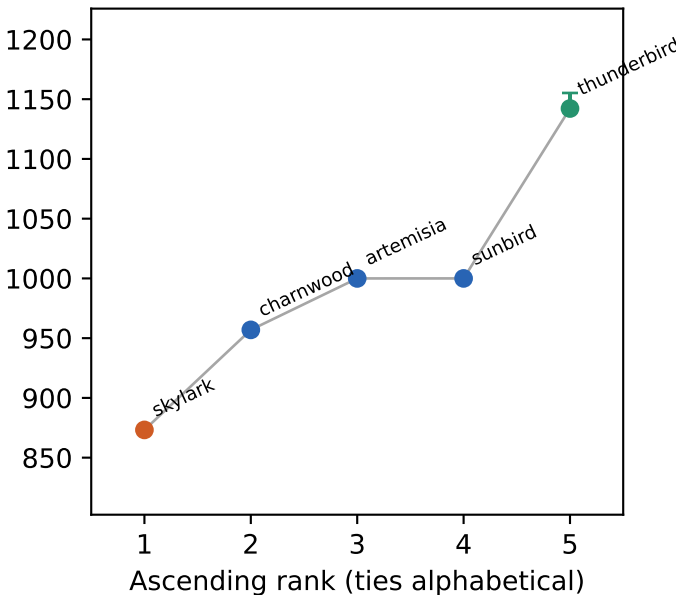
llc misses
