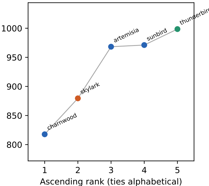
dtlb misses
