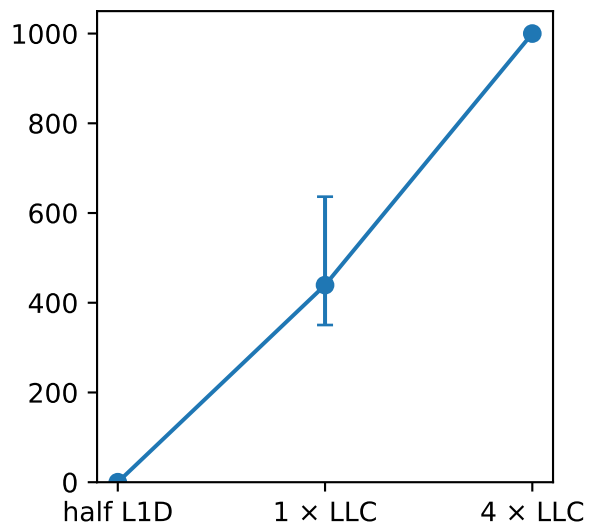
cache-misses
