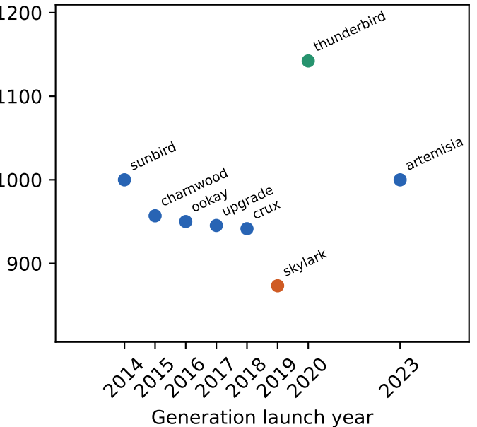
llc misses
