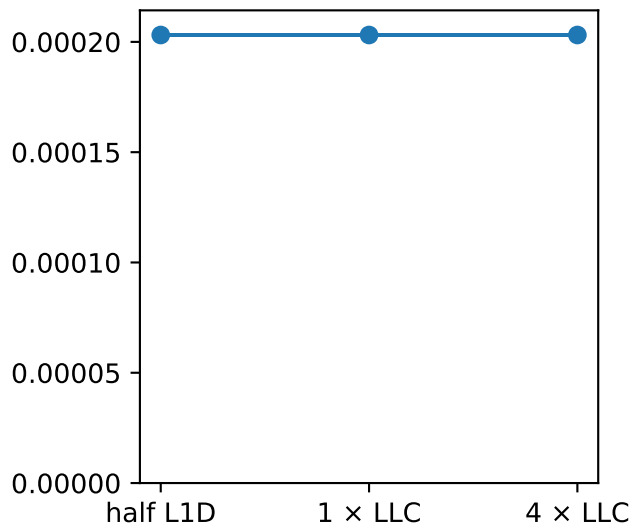
L1-dcache-stores
