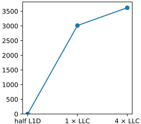
L1-dcache-stores
