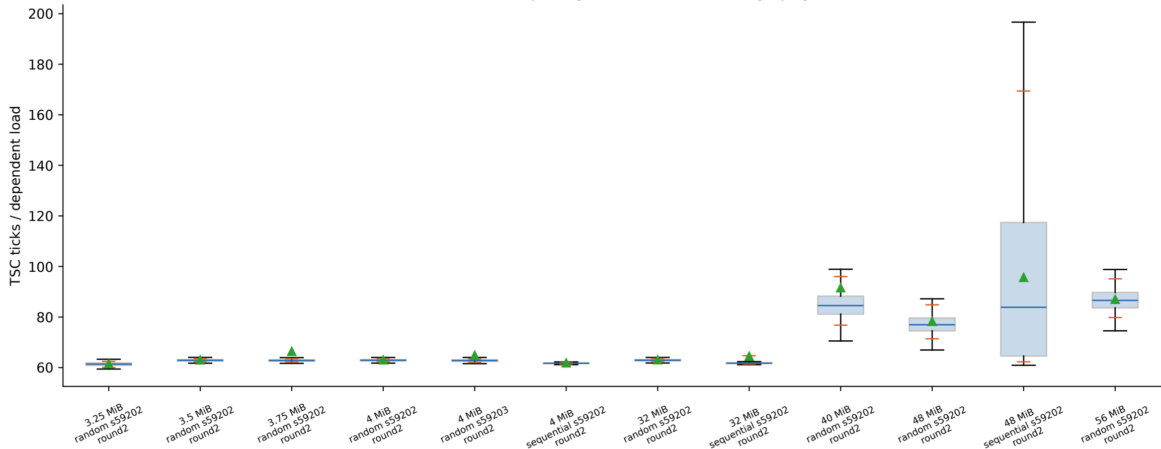
artemisia: 64 B spacing, 256 loads/batch, huge pages
