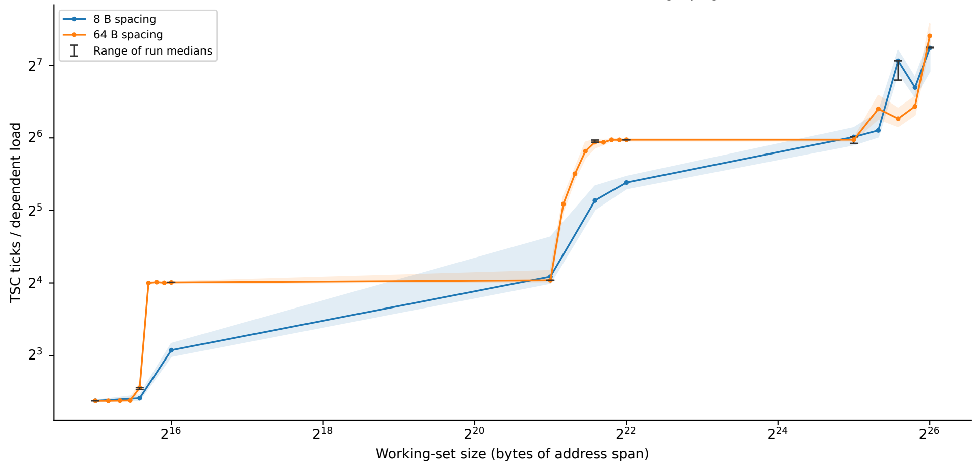
artemisia: random chains, 256 loads/batch, huge pages
