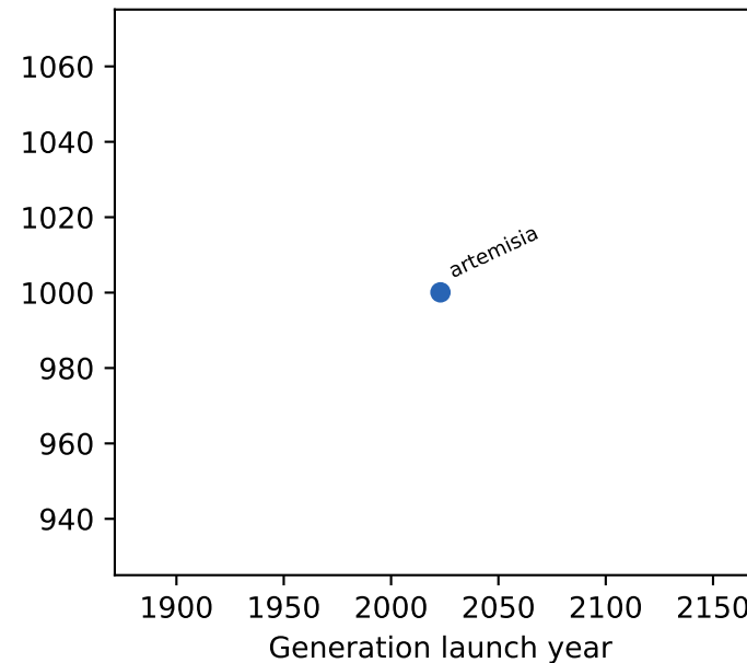
l1c misses
