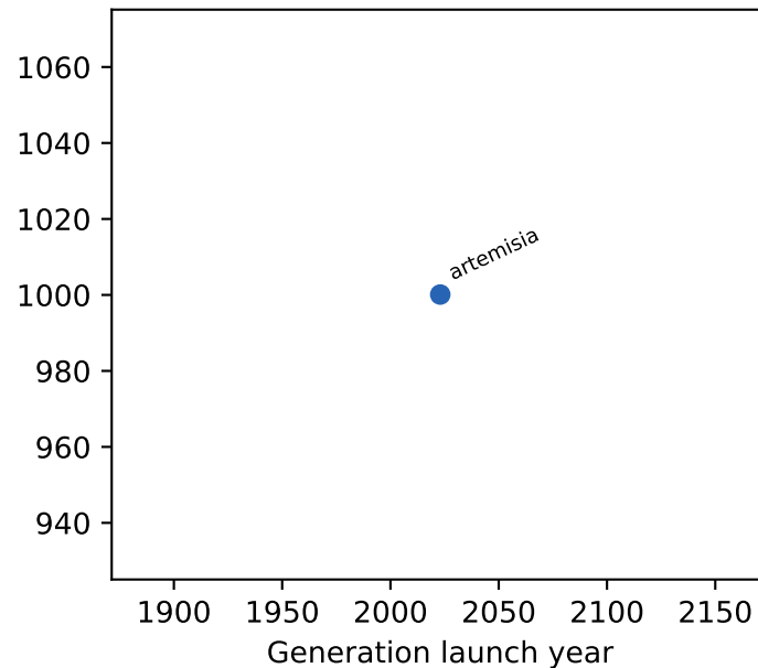
l1c loads
