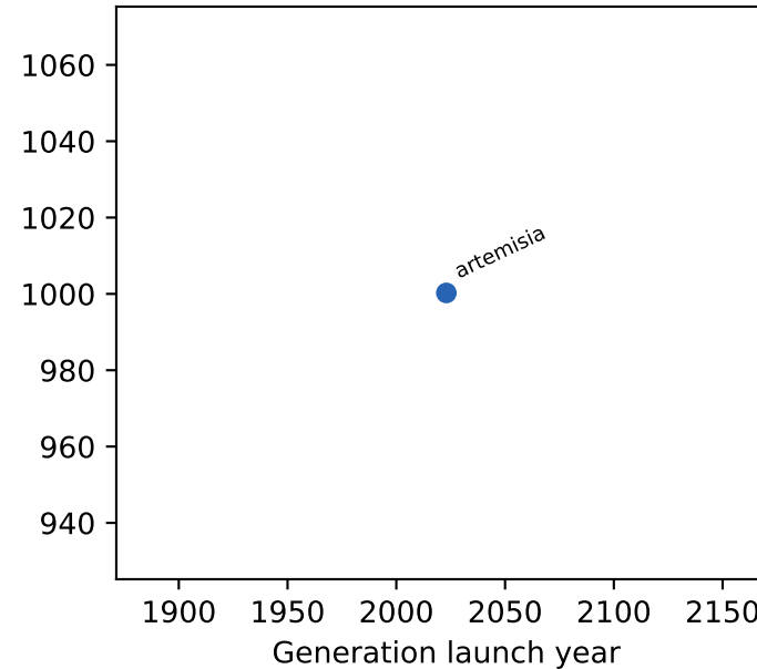
l1c misses
