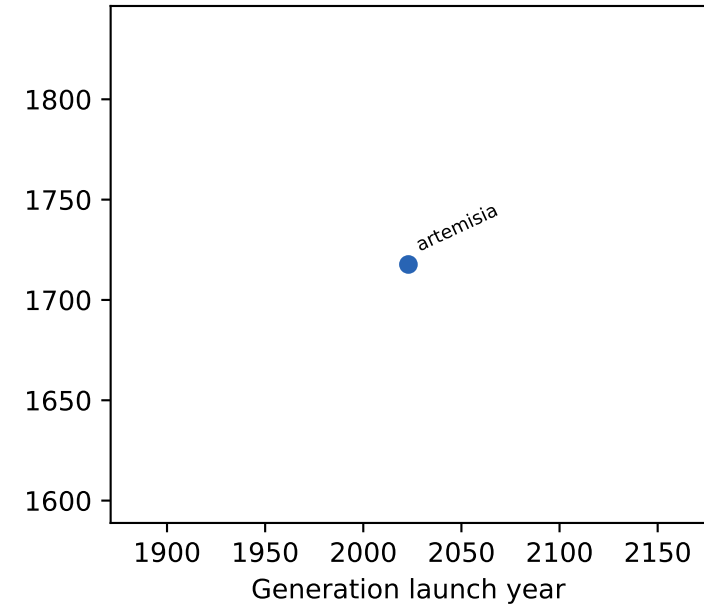
dtlb misses
