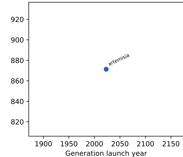
dtlb misses
