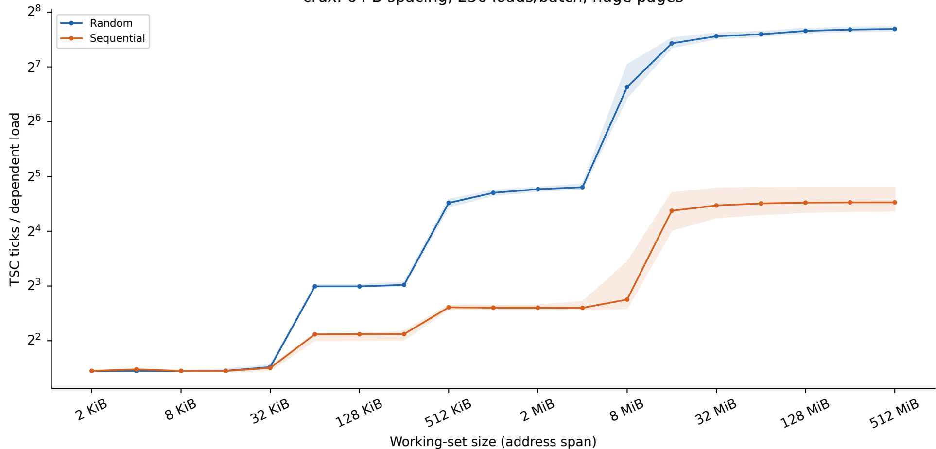
crux: 64 B spacing, 256 loads/batch, huge pages
