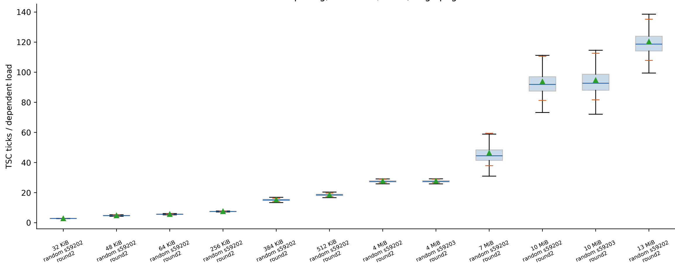
crux: 8 B spacing, 256 loads/batch, huge pages
