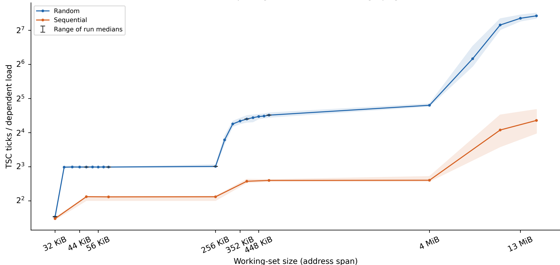
crux: 64 B spacing, 256 loads/batch, huge pages
