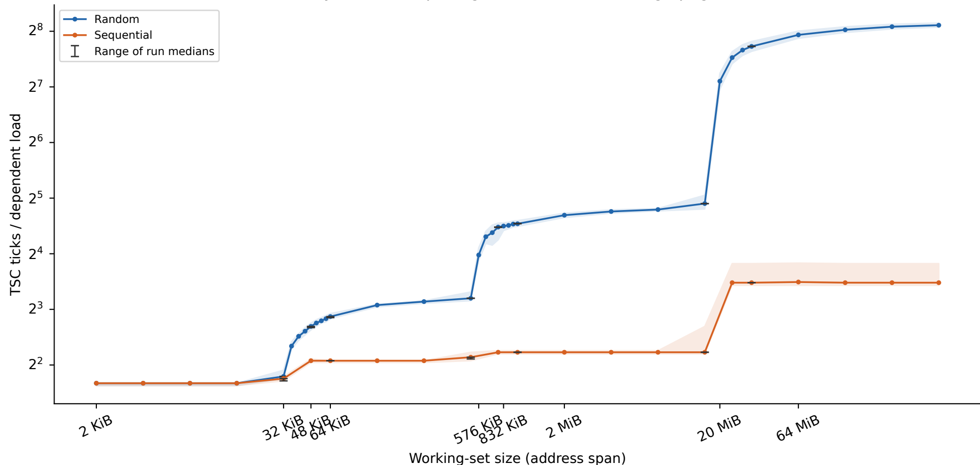
skylark: 64 B spacing, 256 loads/batch, huge pages
