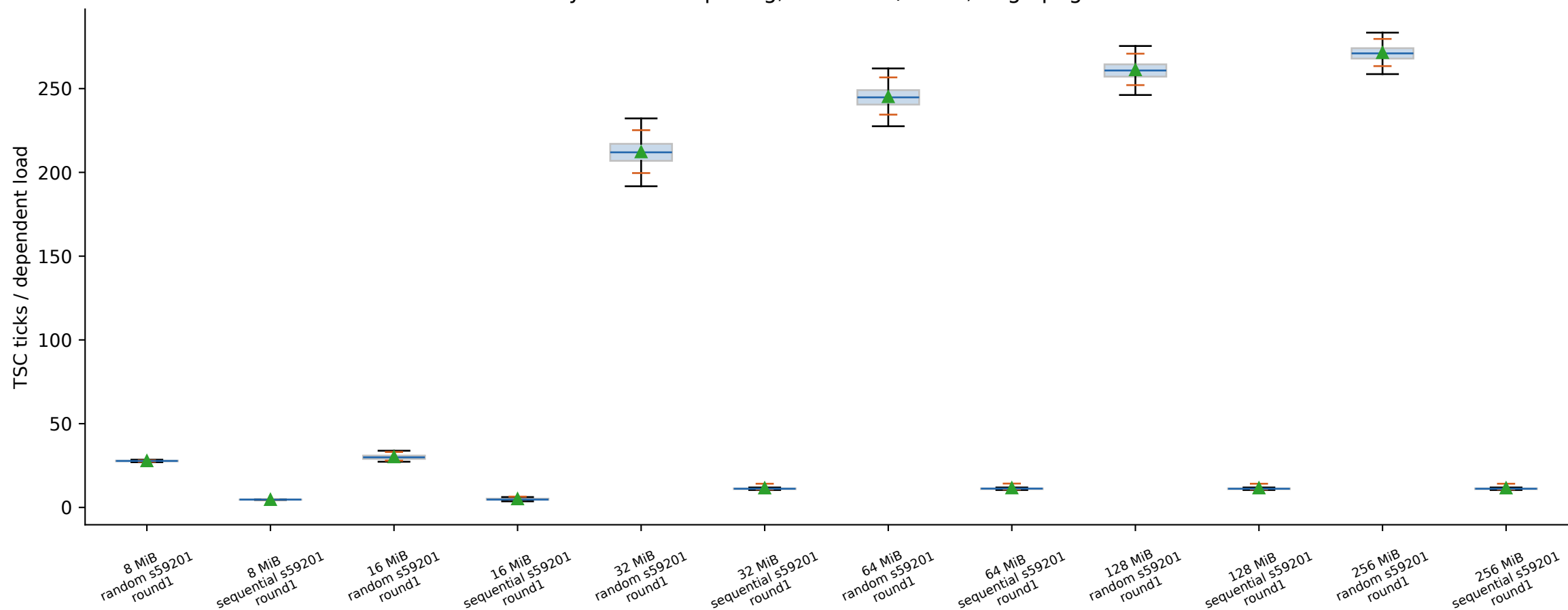
skylark: 64 B spacing, 256 loads/batch, huge pages
