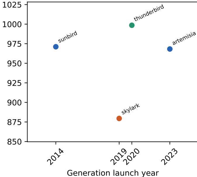
dtlb misses
