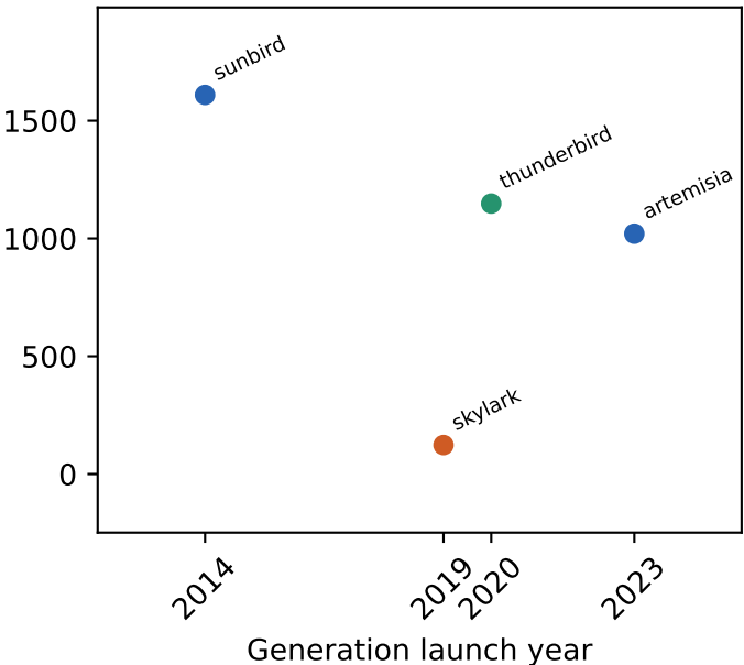
llc loads
