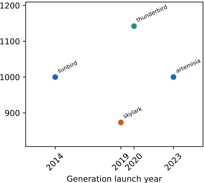
llc misses
