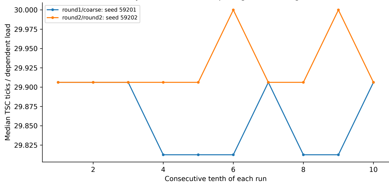
skylark: 16 MiB, 64 B spacing, N=256, huge
