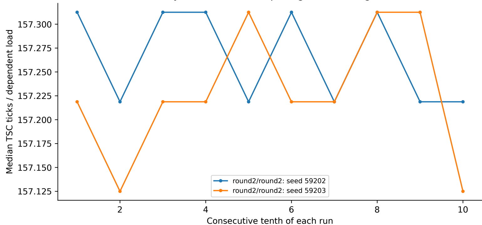
skylark: 32 MiB, 8 B spacing, N=256, huge
