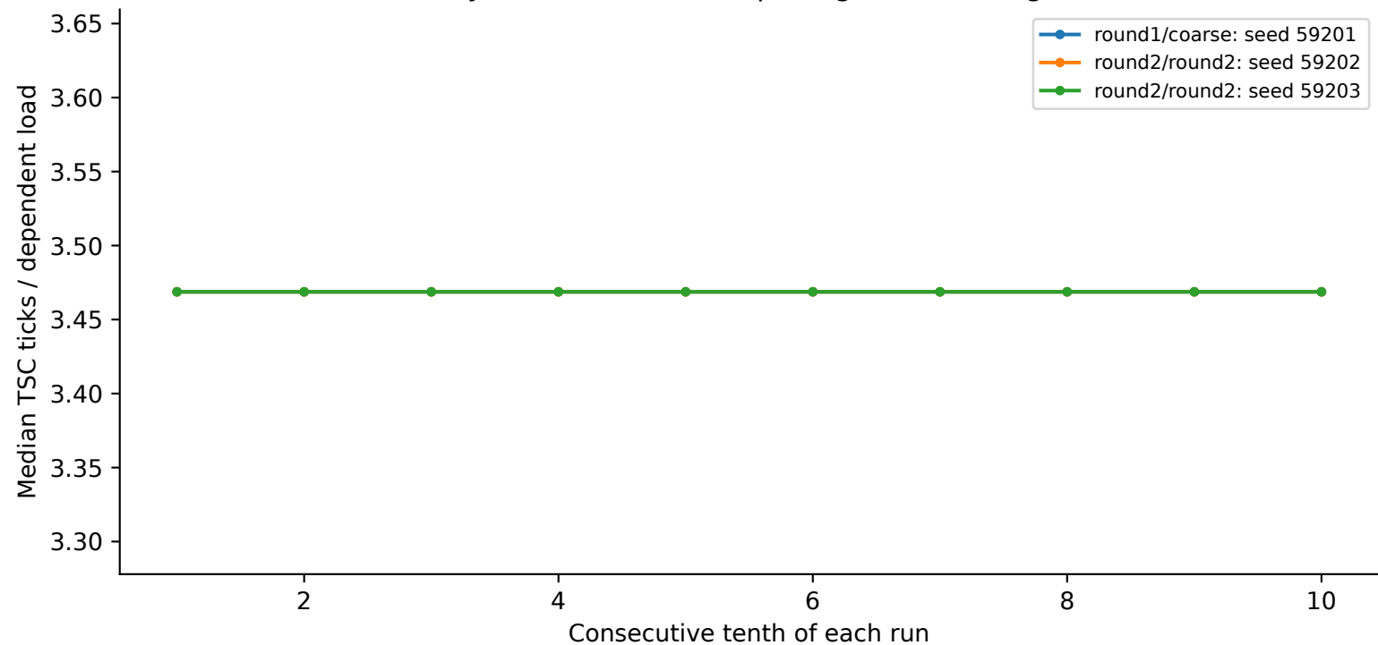
skylark: 32 KiB, 64 B spacing, N=256, huge
