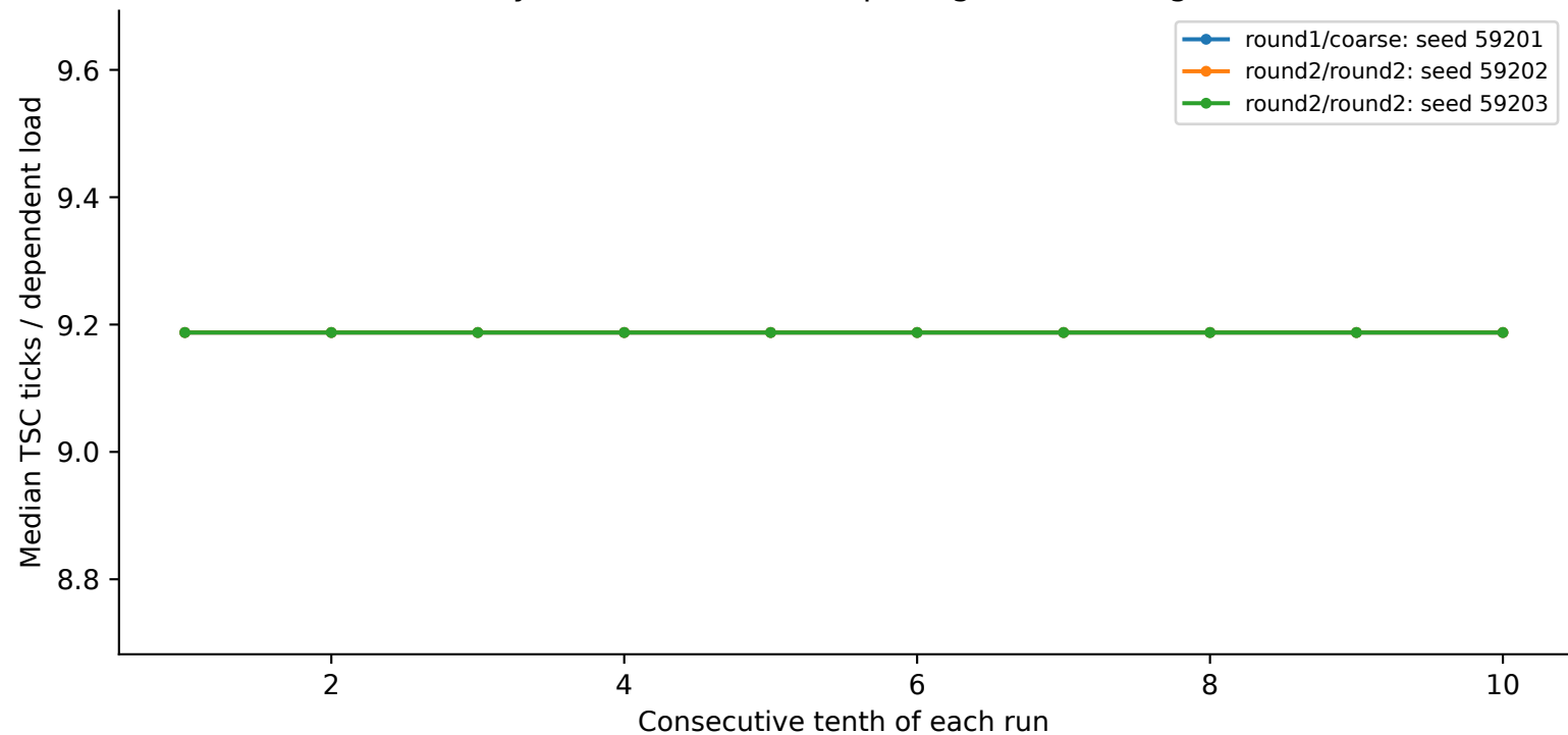
skylark: 512 KiB, 64 B spacing, N=256, huge
