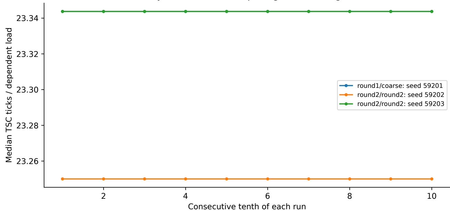
skylark: 1 MiB, 64 B spacing, N=256, huge
