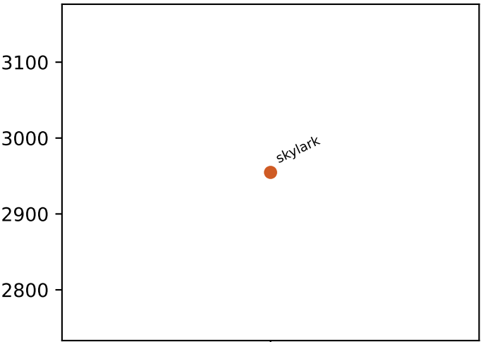
cache references
