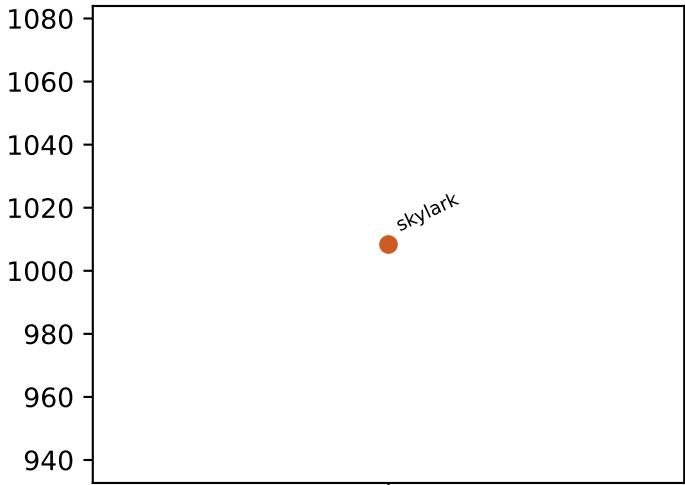
l1 misses
