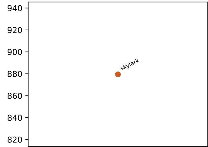
dtlb misses
