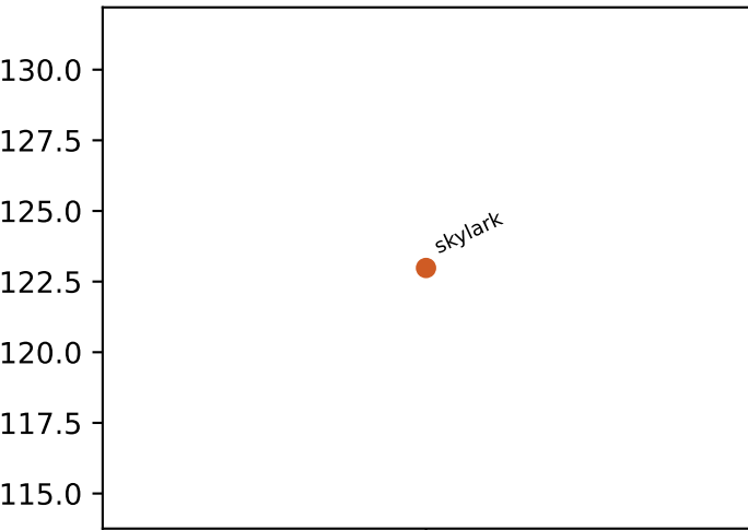
llc loads
