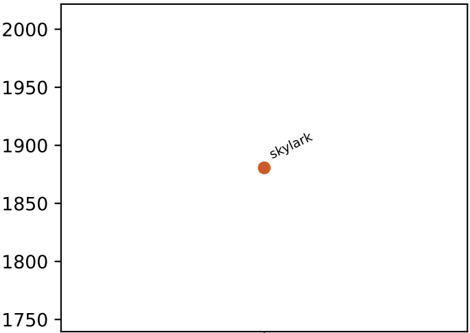
l1 loads
