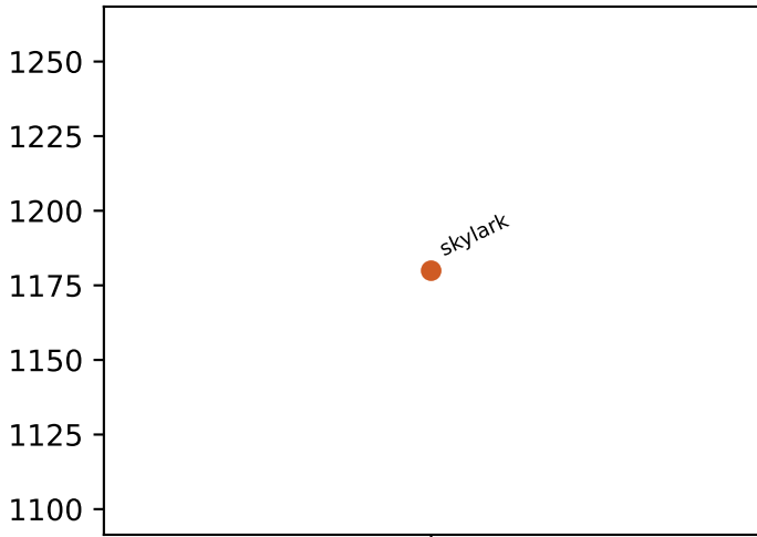
cache misses
