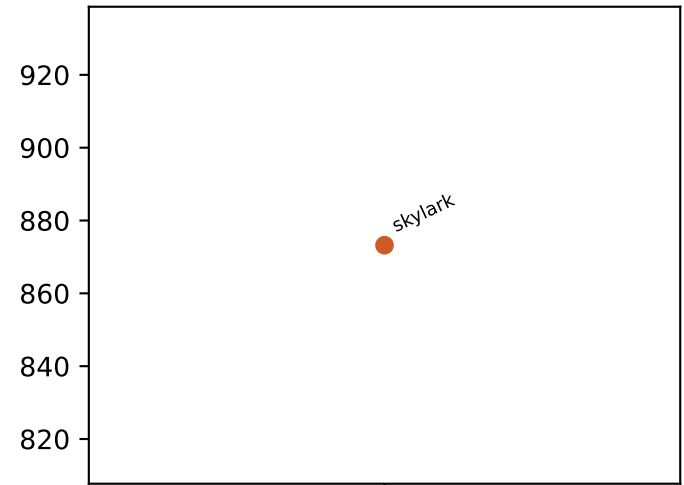
llc misses
