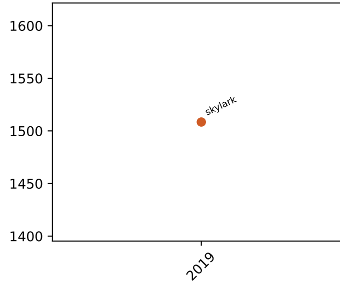
l1 loads
