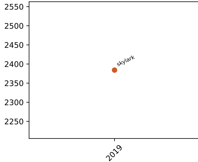
cache references
