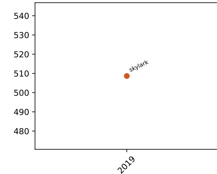
dtlb misses
