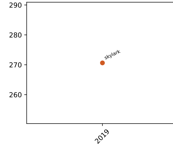
l1c misses
