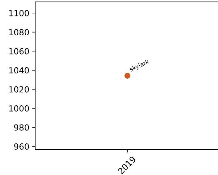
l1 misses
