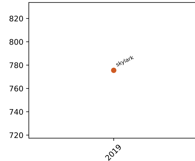
l1c loads
