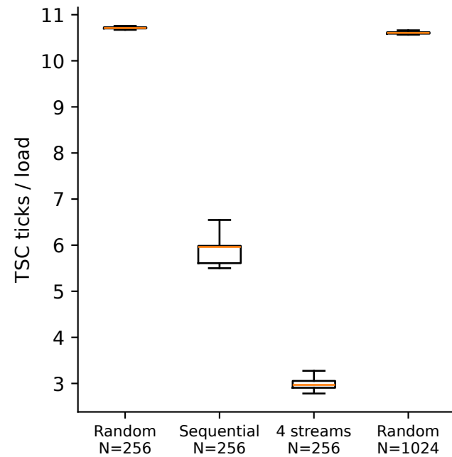
L2 method controls
