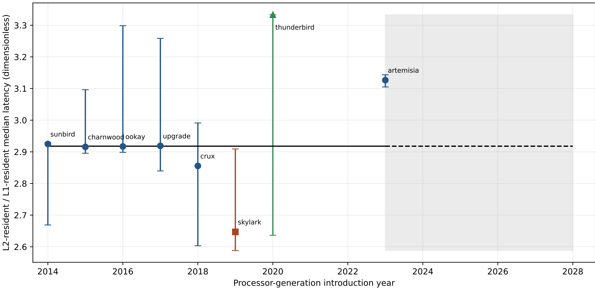
Patel-Wu Relative Cache Latency Law
