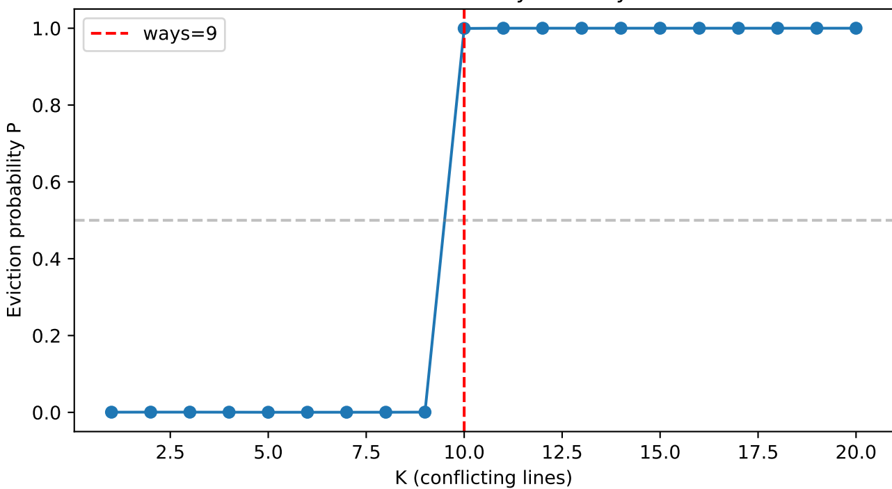
LLC - associativity \approx 9-way
