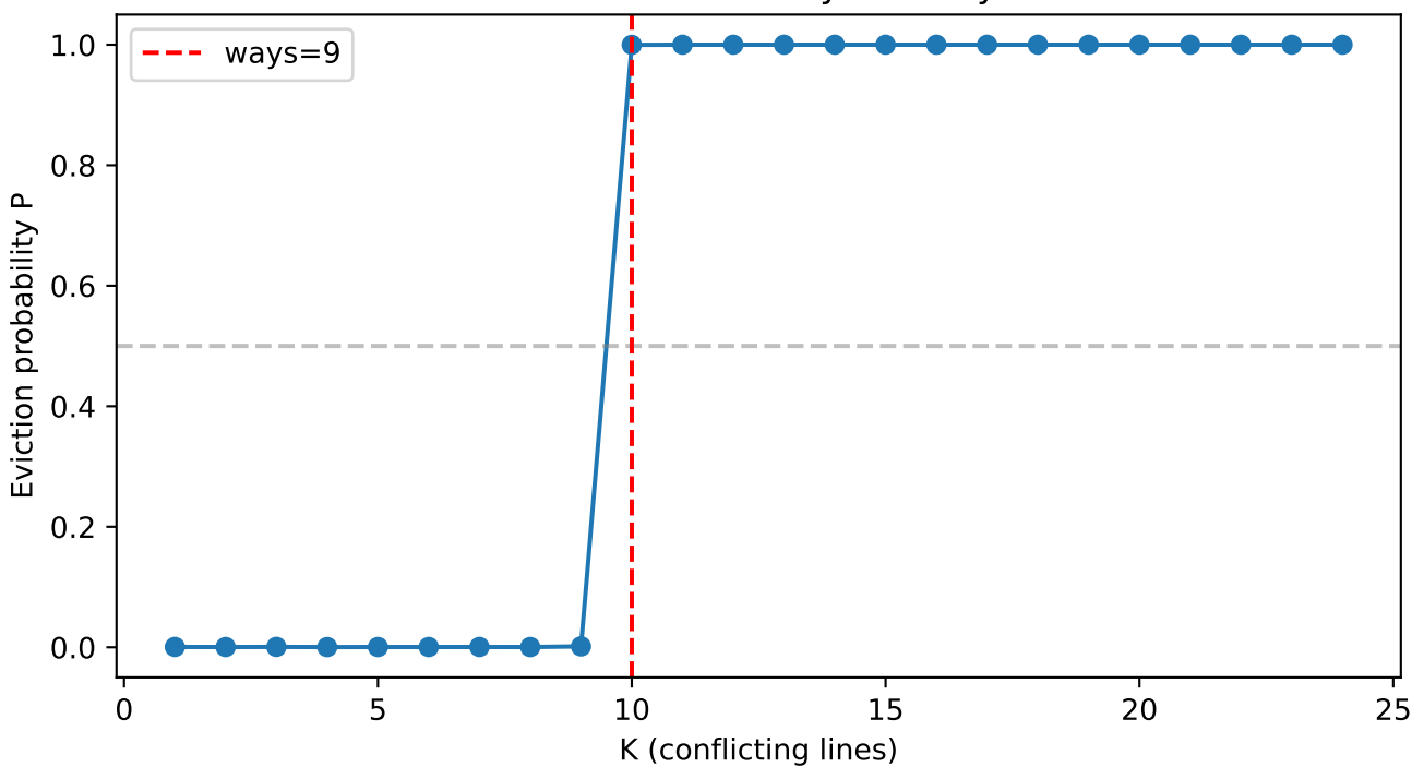
LLC - associativity \approx 9-way
