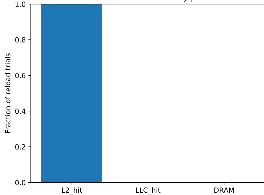
crux: T reload after LLC-only pressure
