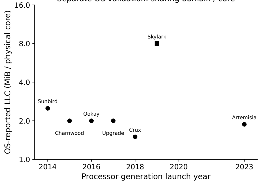
Separate OS validation: sharing domain / core
