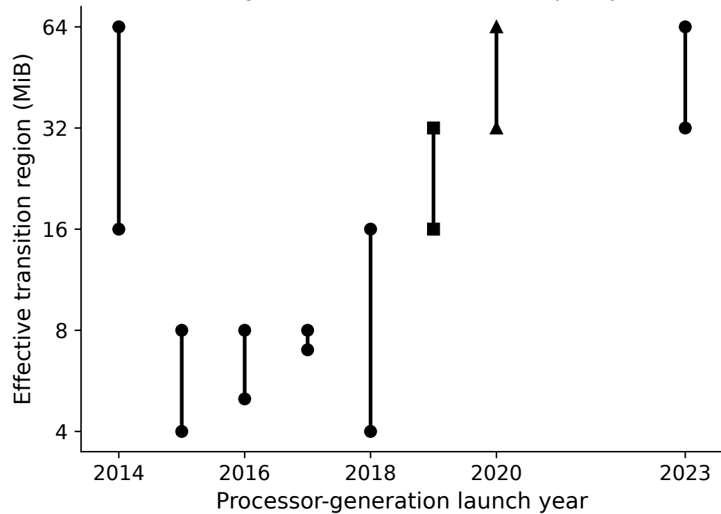
Timing evidence: no exact LLC capacity
