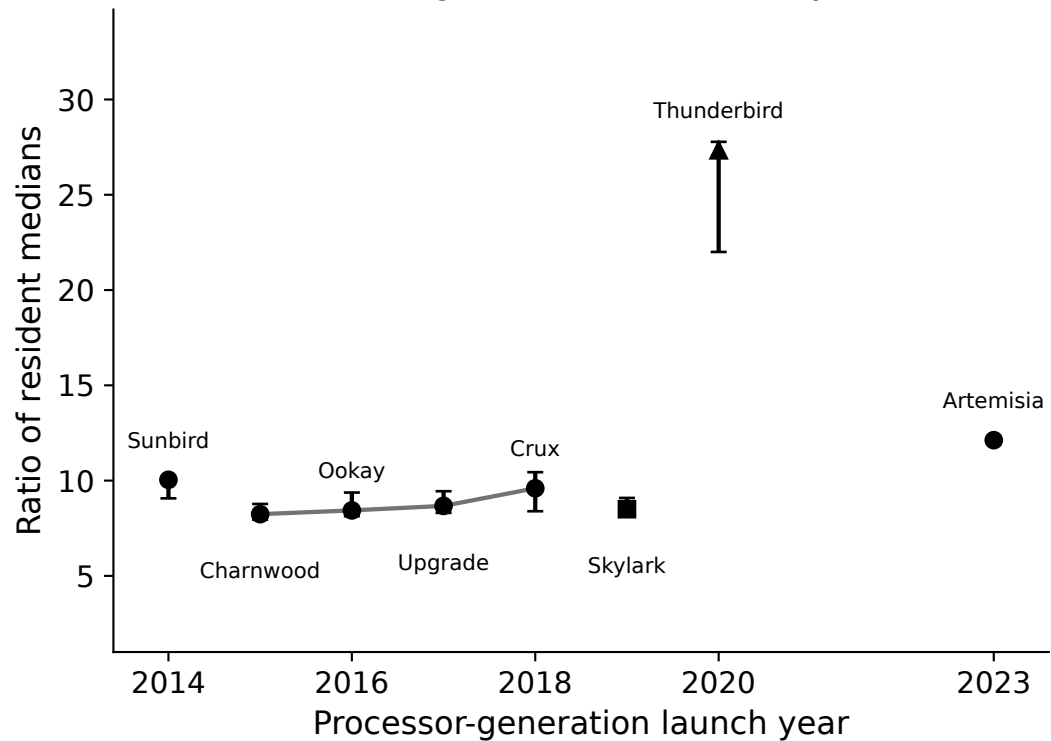
LLC-region / L1 relative latency
