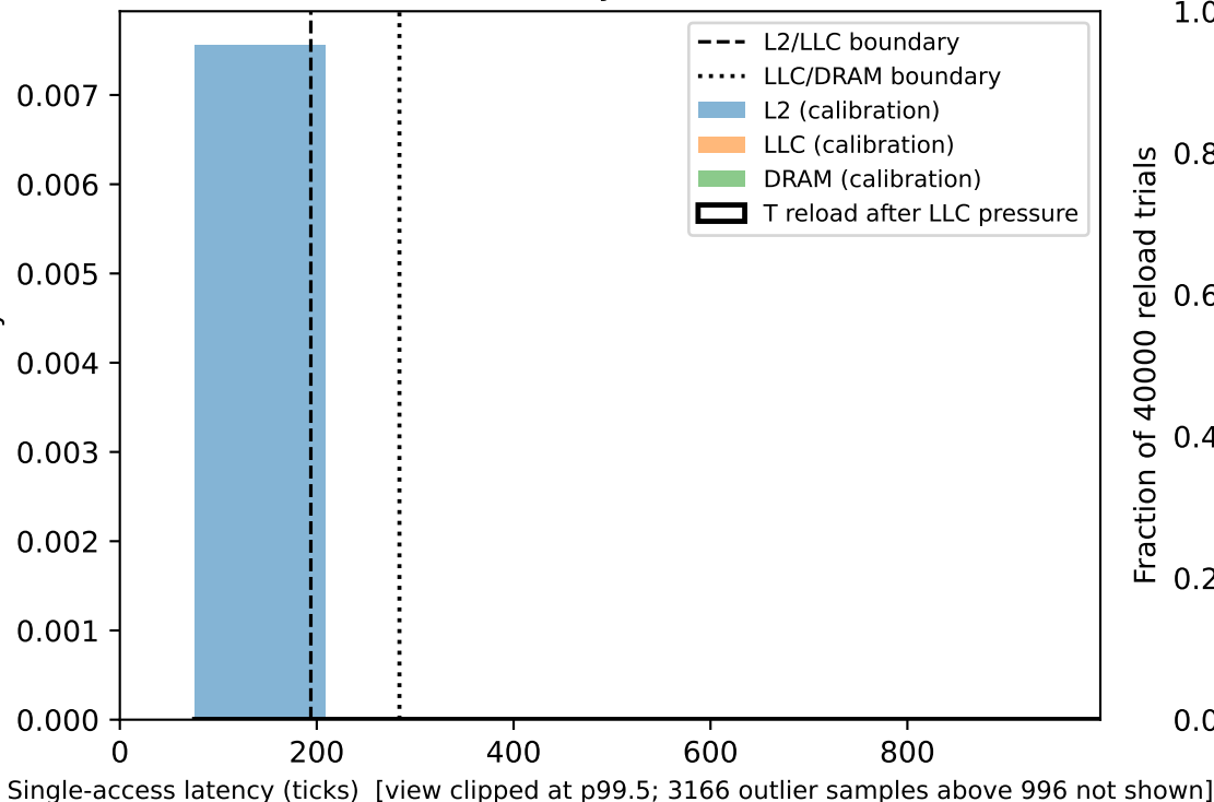
sunbird: reload latency vs. calibrated classes
