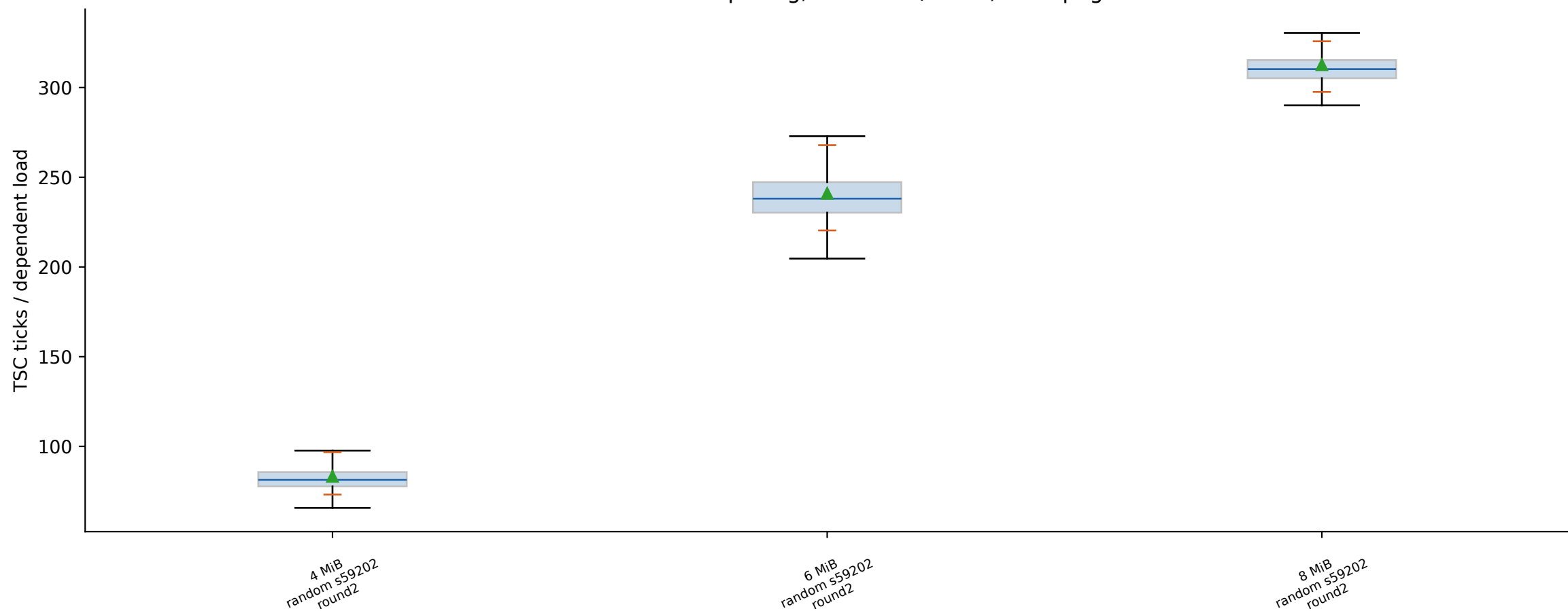
charnwood: 64 B spacing, 256 loads/batch, base pages
