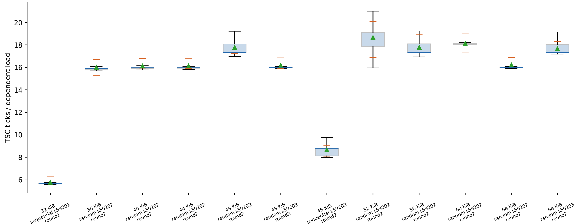
charnwood: 64 B spacing, 256 loads/batch, huge pages
