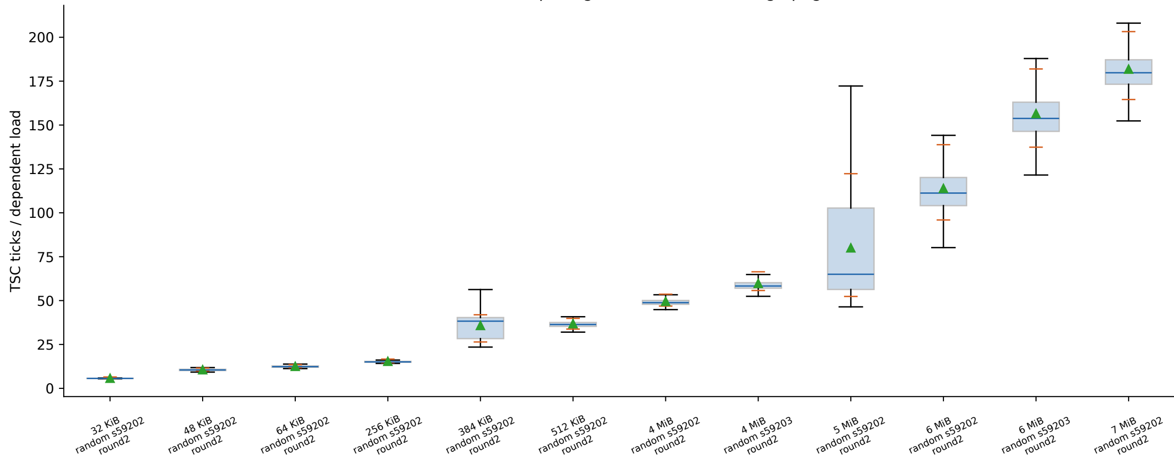
charnwood: 8 B spacing, 256 loads/batch, huge pages
