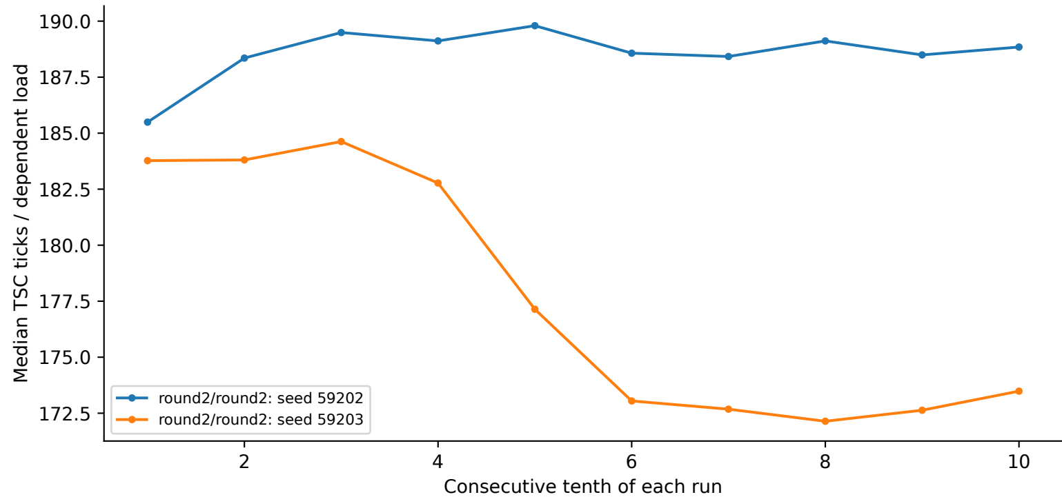
charnwood: 8 MiB, 8 B spacing, N=256, huge
