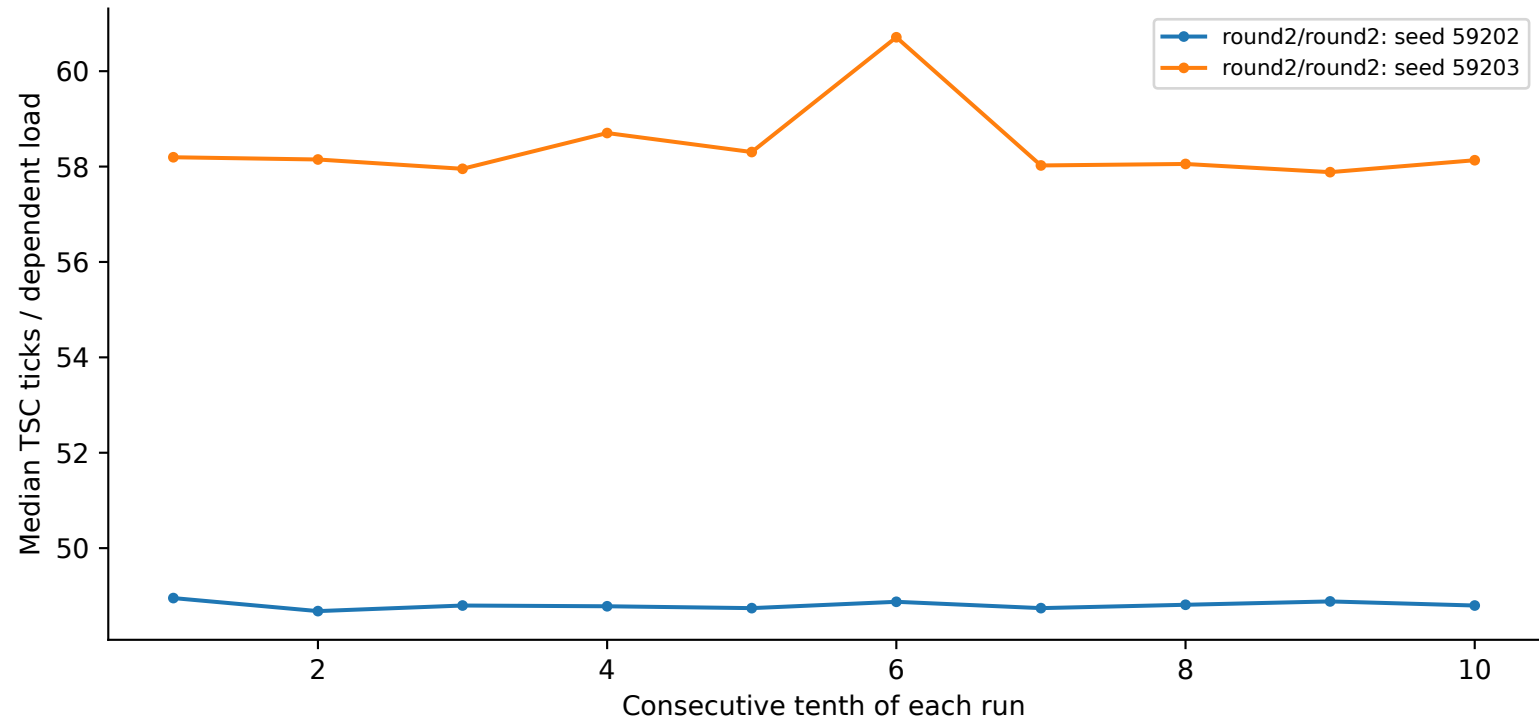
charnwood: 4 MiB, 8 B spacing, N=256, huge
