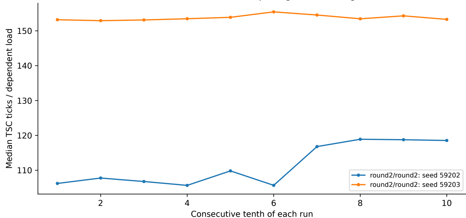
charnwood: 6 MiB, 8 B spacing, N=256, huge
