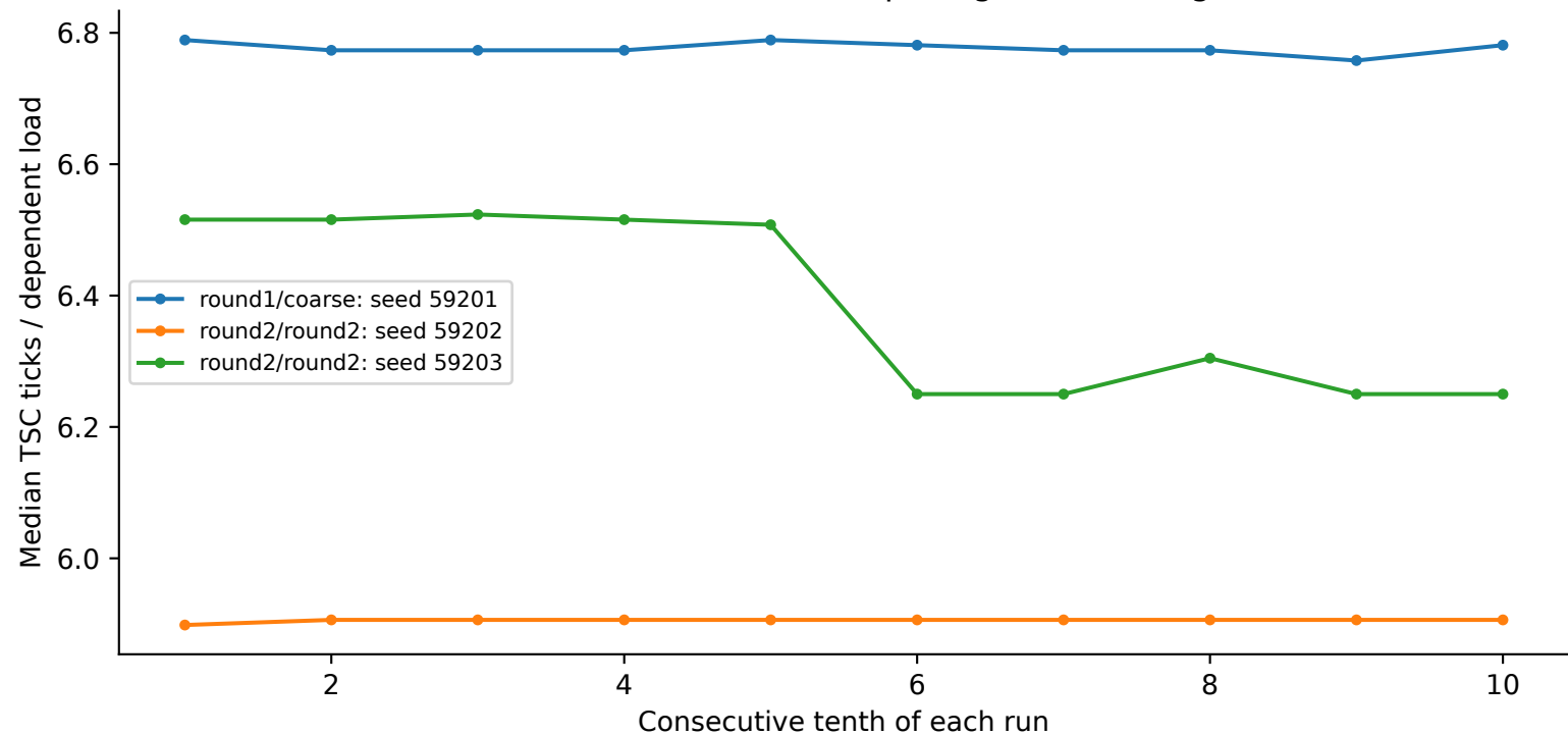
charnwood: 32 KiB, 64 B spacing, N=256, huge
