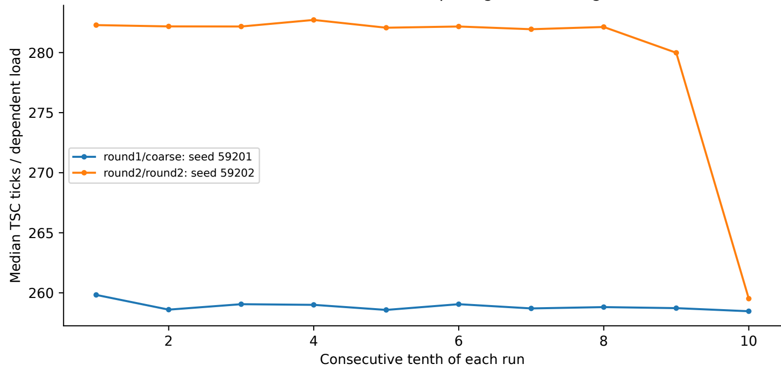
charnwood: 8 MiB, 64 B spacing, N=256, huge
