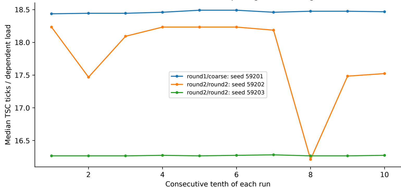
charnwood: 256 KiB, 64 B spacing, N=256, huge
