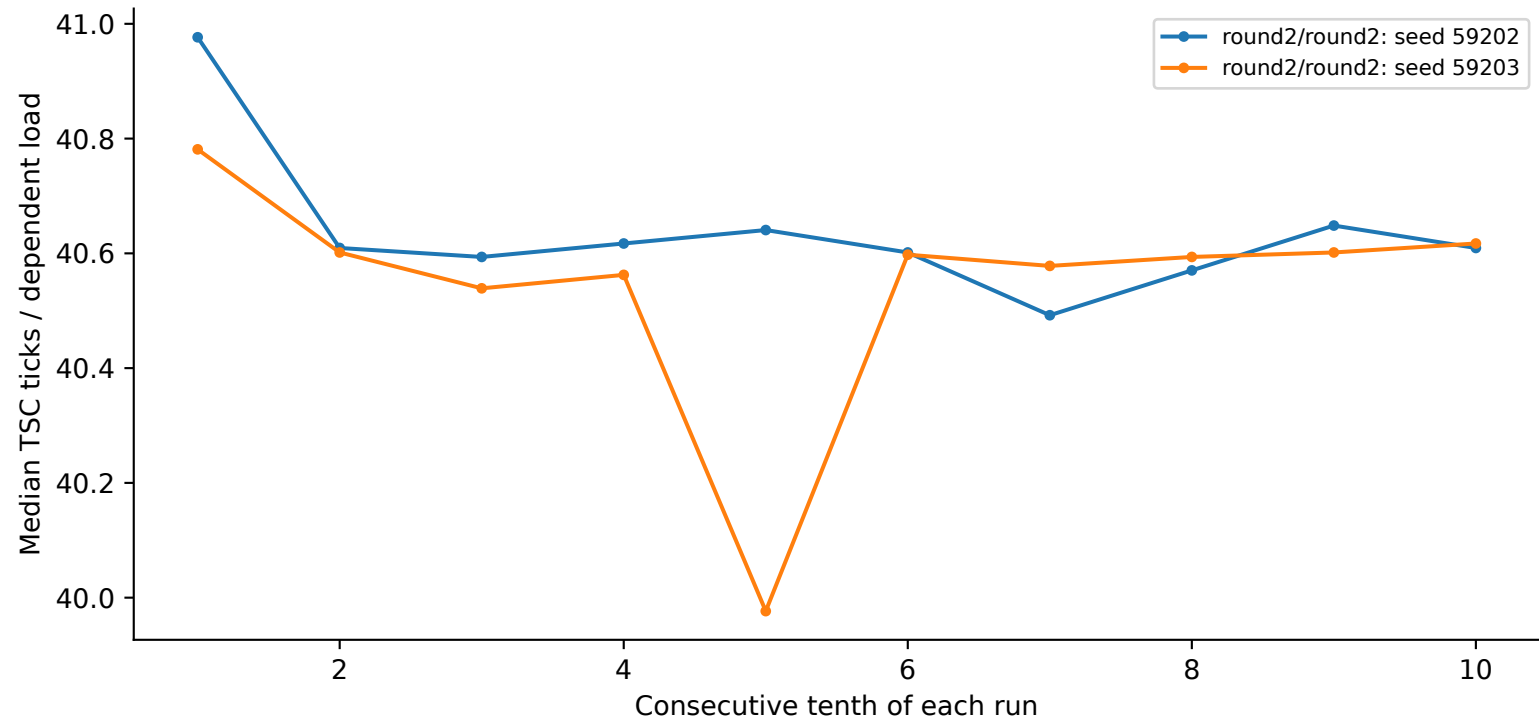
charnwood: 384 KiB, 64 B spacing, N=256, huge
