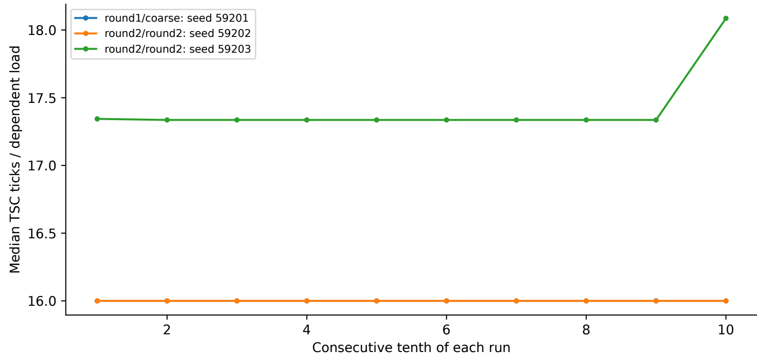
charnwood: 64 KiB, 64 B spacing, N=256, huge
