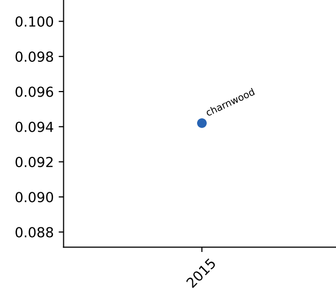
l1 misses
