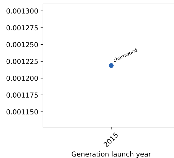
l1c misses
