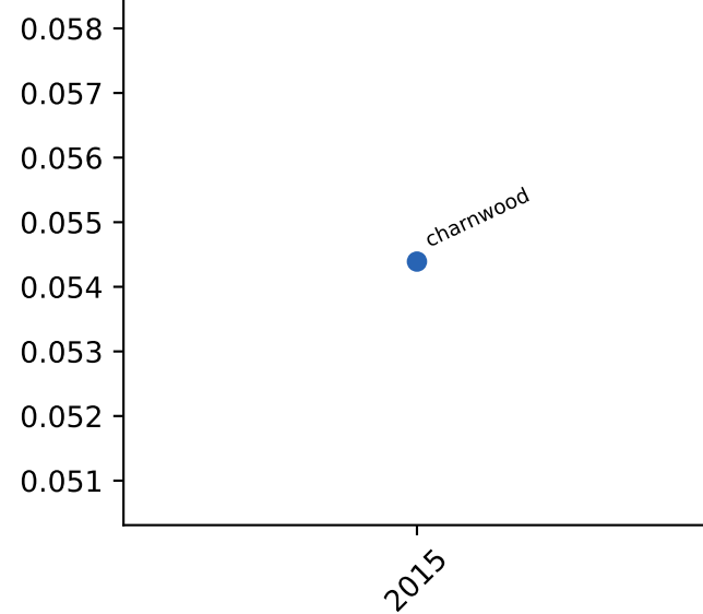
cache references
