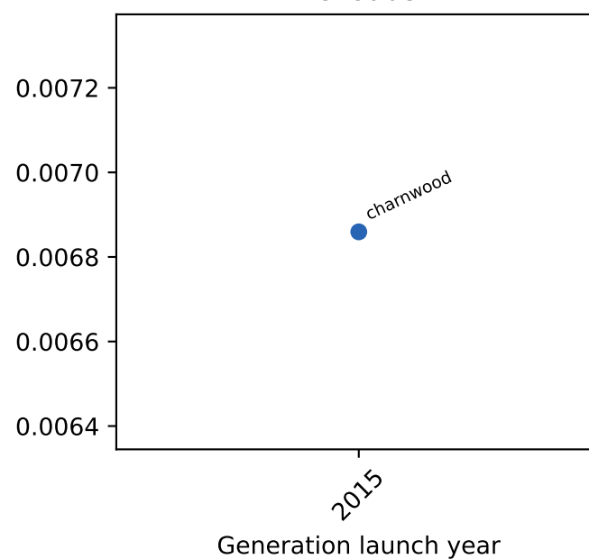
l1c loads
