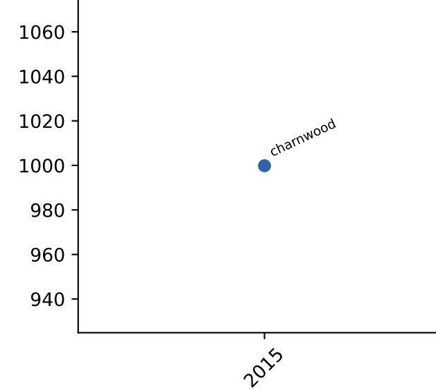
l1 loads
