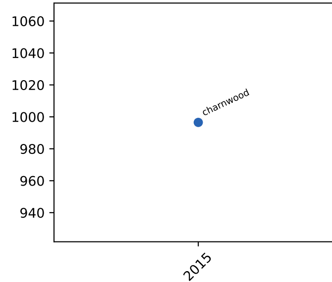
l1 loads
