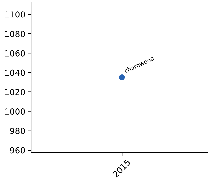
cache misses
