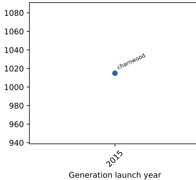
l1c loads
