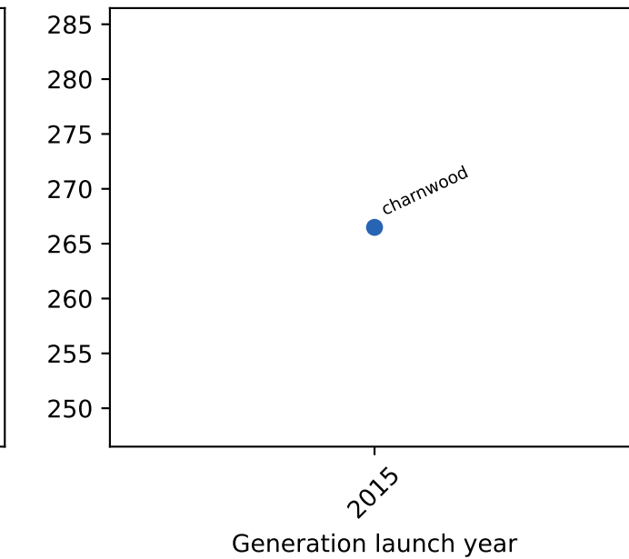
dtlb misses
