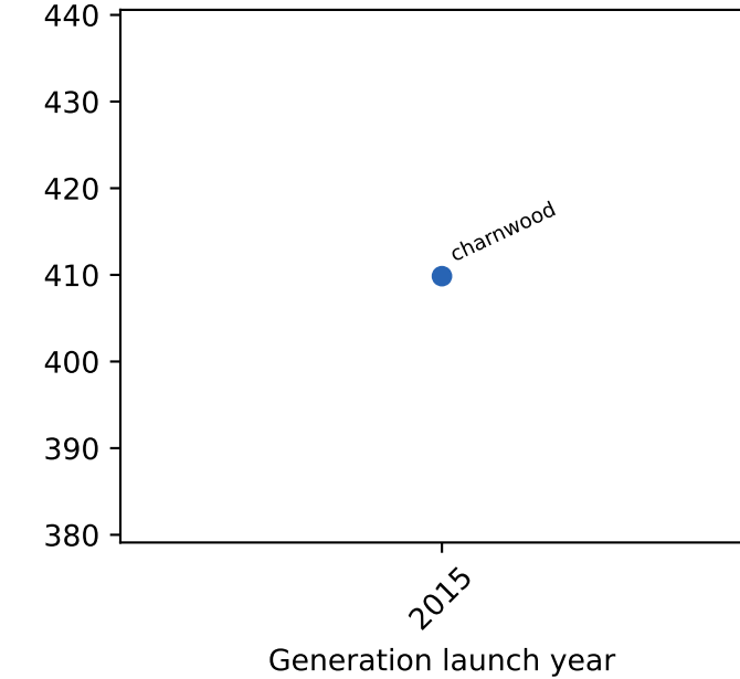
l1c misses
