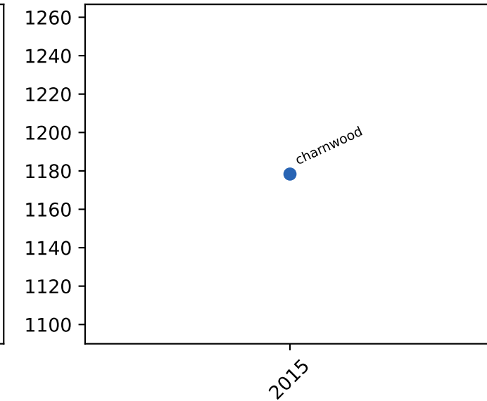
l1 misses
