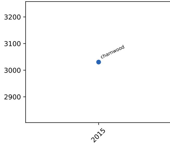
cache references
