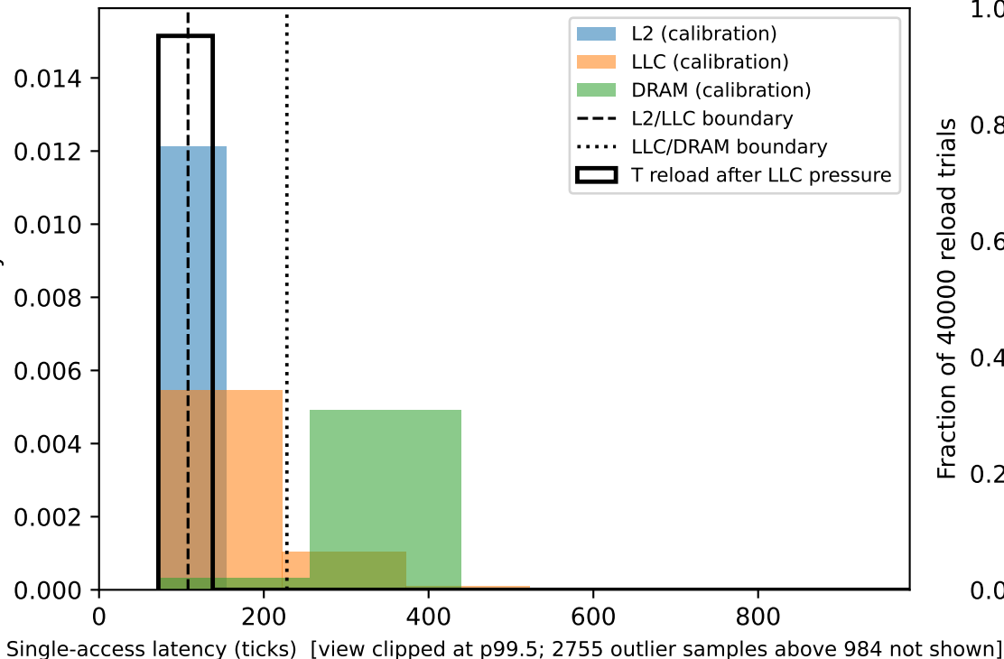
skylark: reload latency vs. calibrated classes
