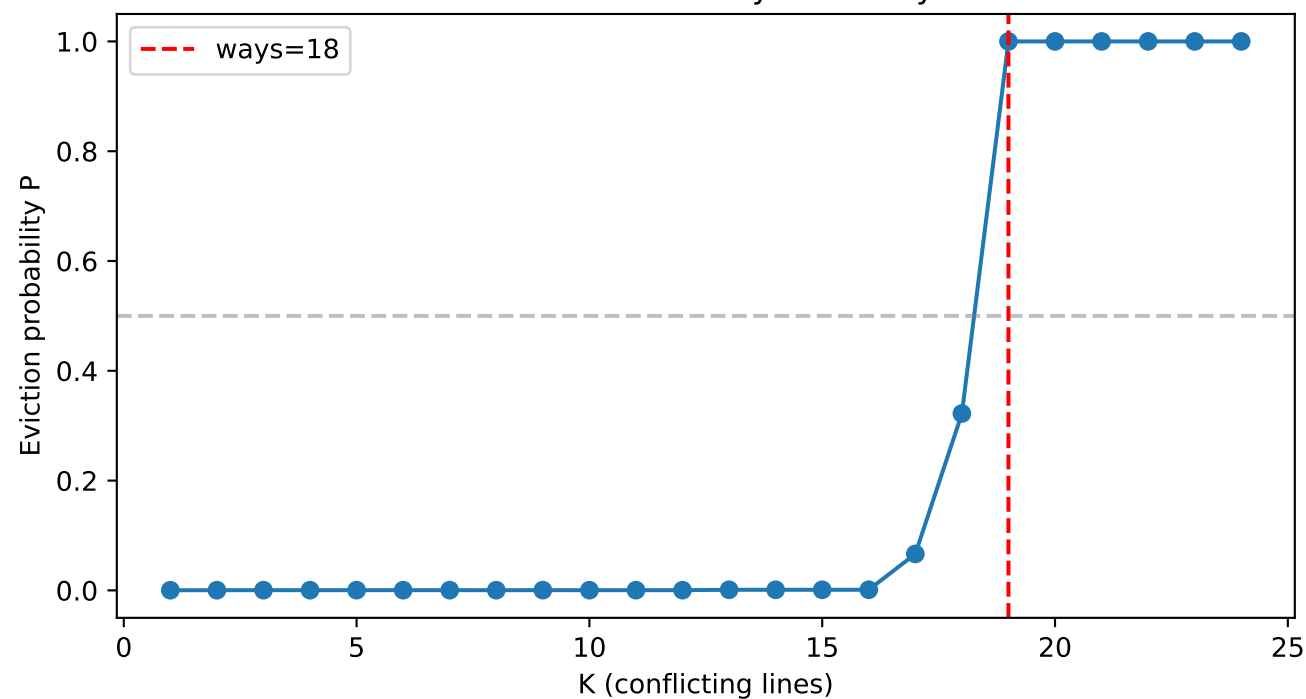
LLC - associativity \approx 18-way
