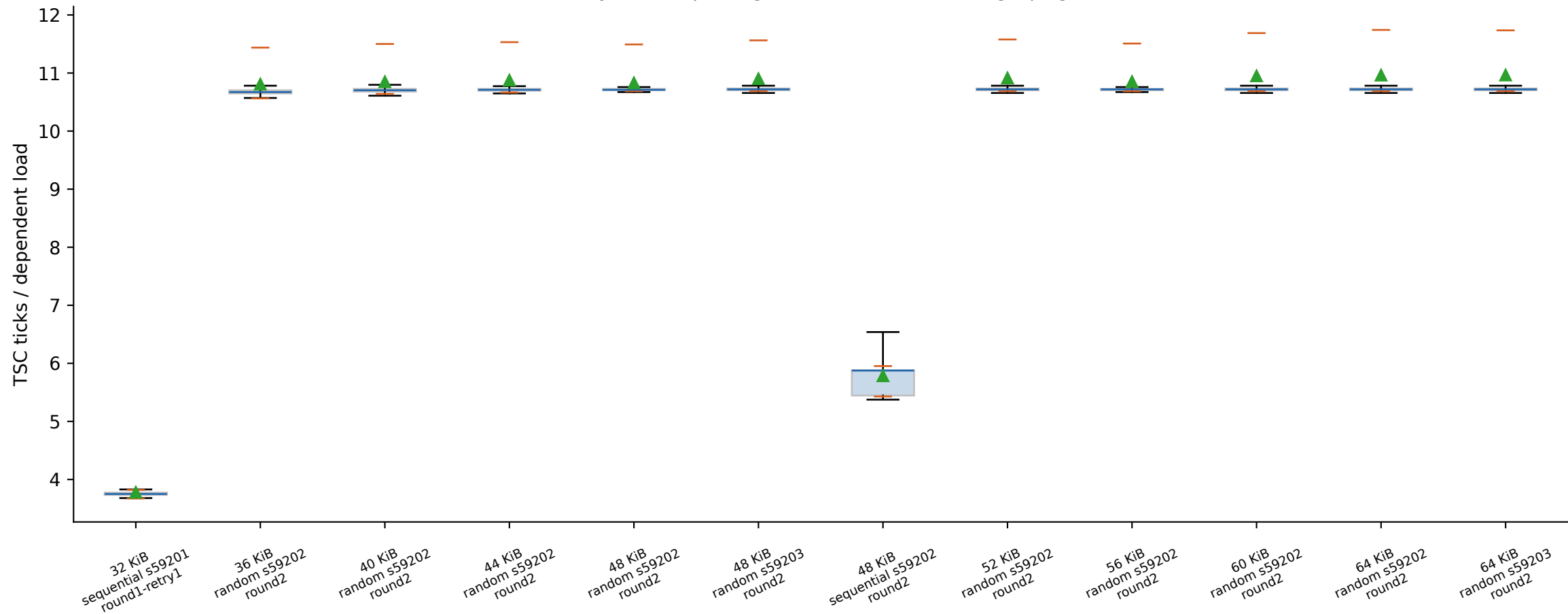
ookay: 64 B spacing, 256 loads/batch, huge pages
