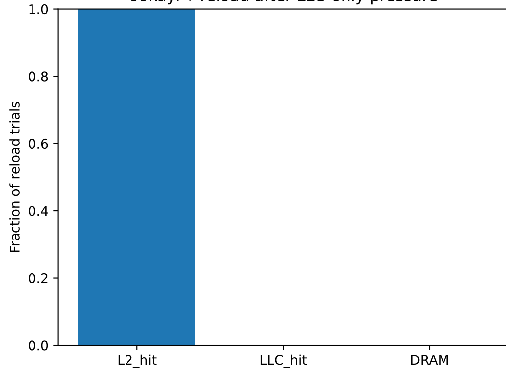
ookay: T reload after LLC-only pressure
