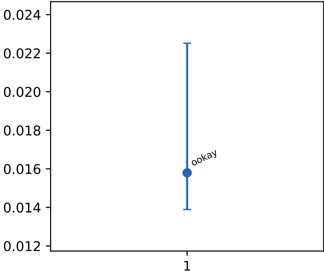
l1c loads
