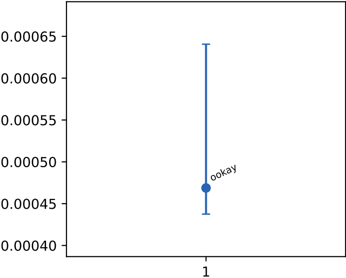
dtlb misses
