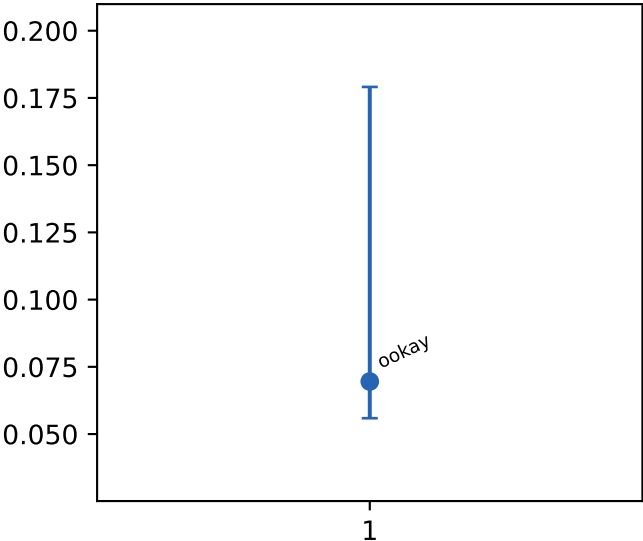
cache references
