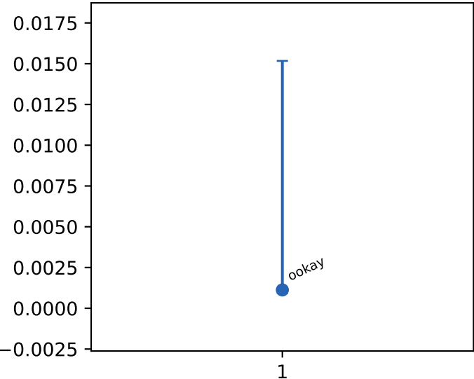
cache misses
