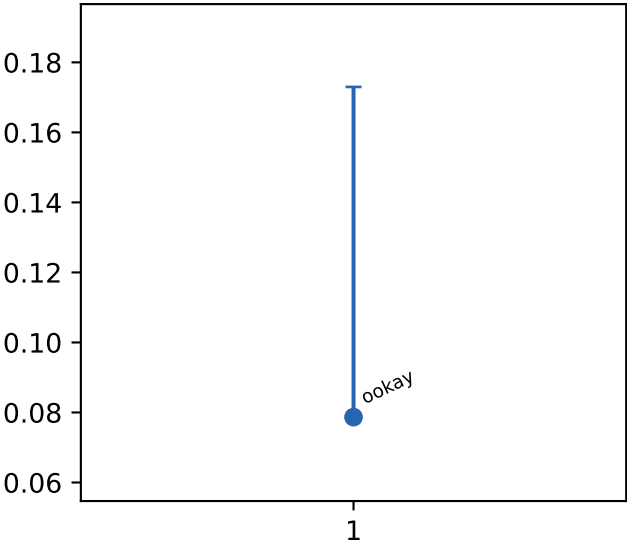
l1 misses
