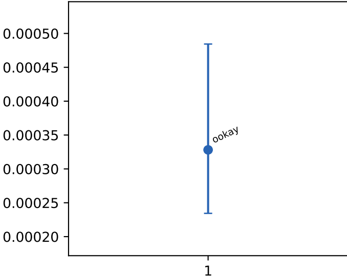
l1c misses
