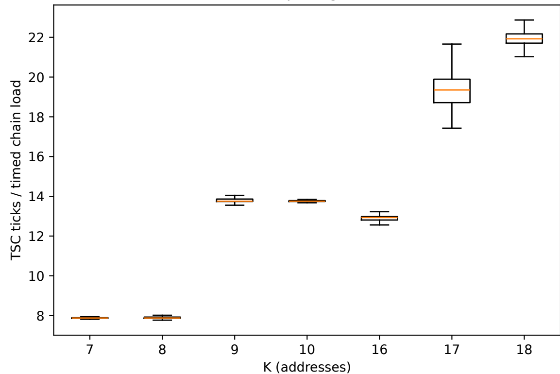
16 KiB address spacing (L2 candidate)
